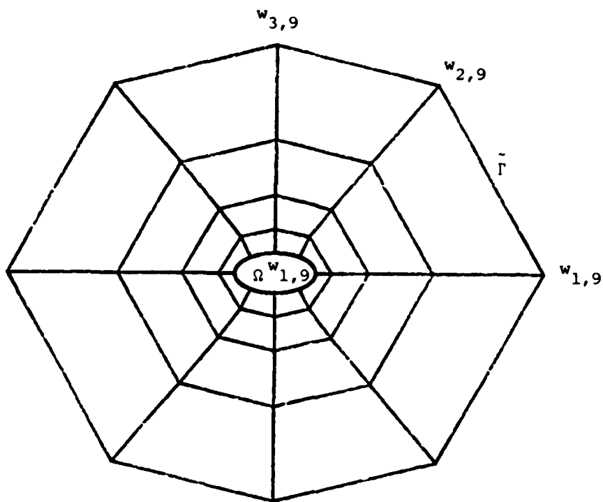
Figure 5.1: 17 basis functions
