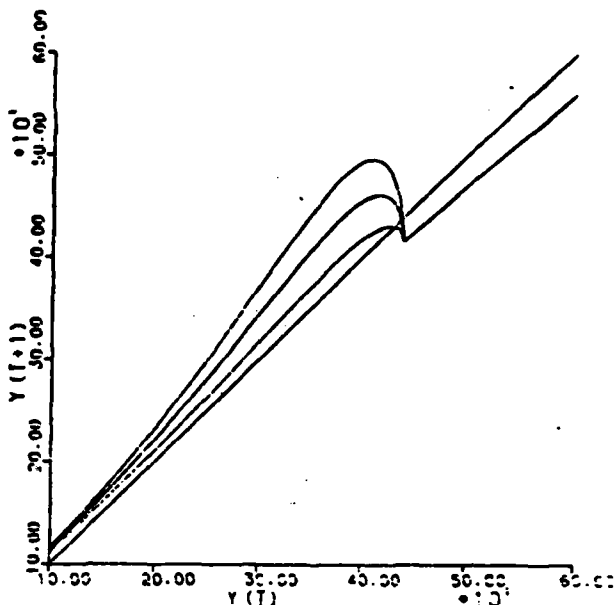
(b) Aggregate Demand for Increasing \mu
