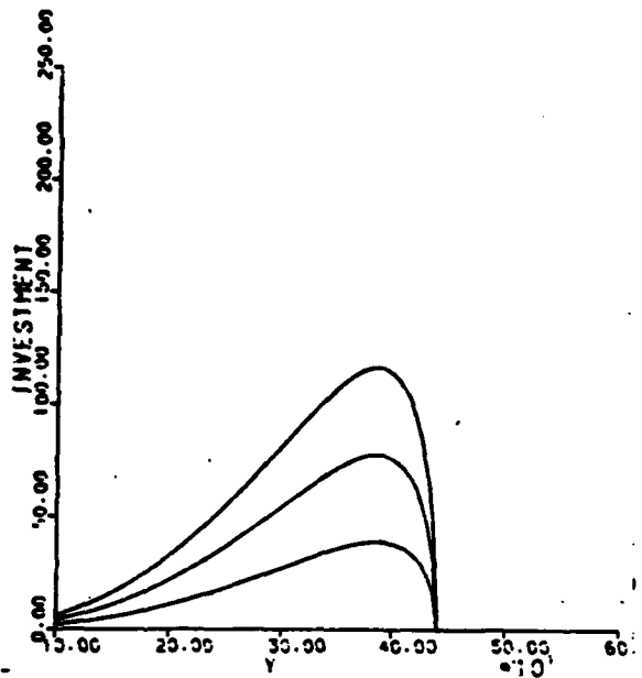
(a) Induced Investment for Increasing \mu
