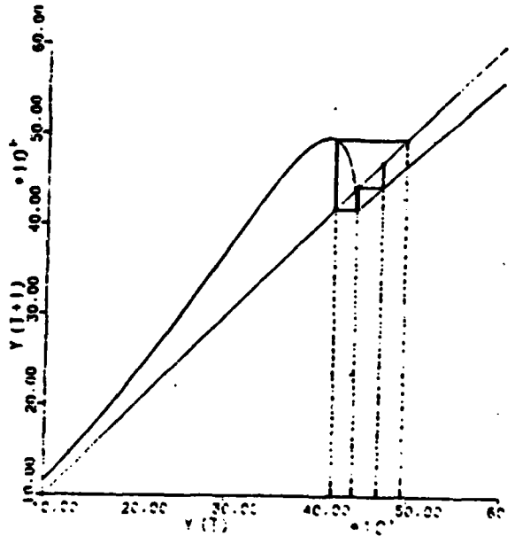
(c) Sufficient Chaos Condition Satisfied
