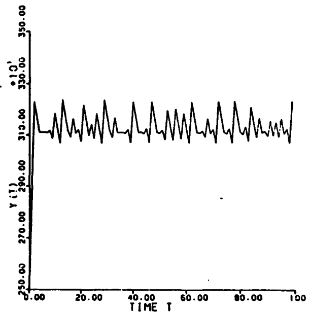
(e) A Chaotic Trajectory
