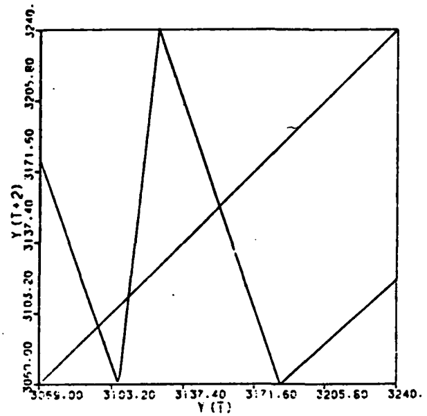
(b) Second Iterate
