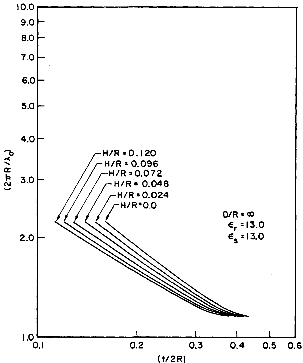
Fig. 5 — Simulation of design geometries for circular disk dielectric (GaAs) resonator on dielectric (GaAs) substrate for this substrates.
