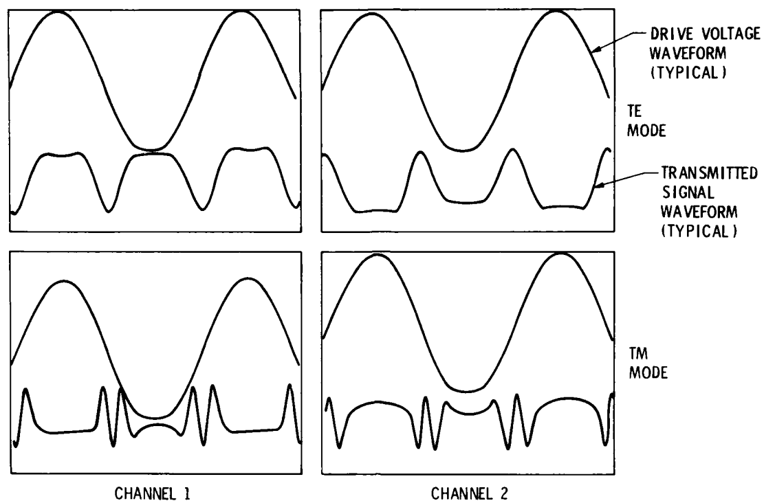
FIGURE 9 WAVEGUIDE COUPLER SINE WAVE RESPONSE
