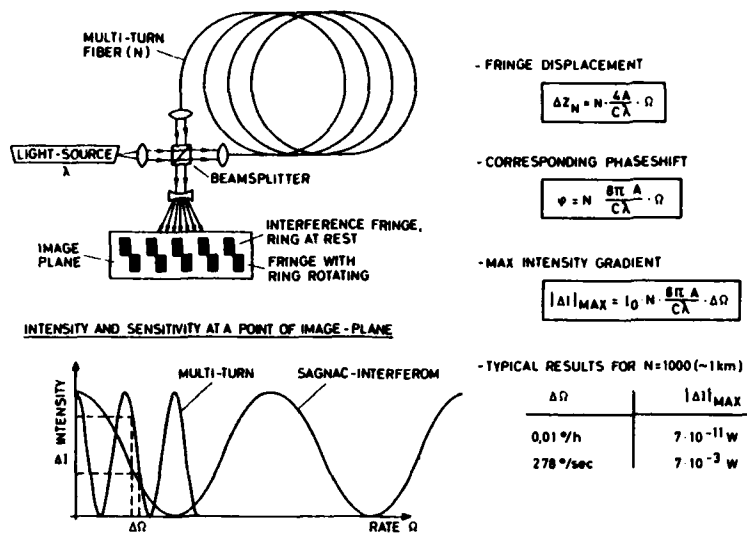
Fig.3-4: MULTI-TURN SAGNAC-INTERFEROMETER (FIBER-OPTIC GYRO)
