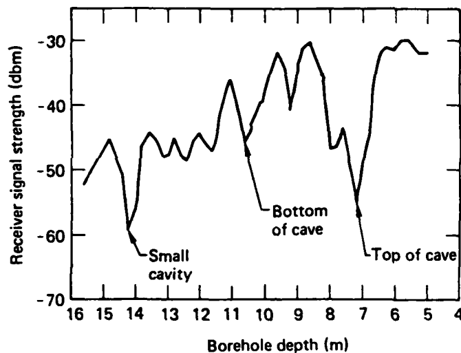
FIG. 10. Plot of high-frequency EM transmission between boreholes C3 and C5 at Medford Caves. The frequency is fixed at 100 MHz.
