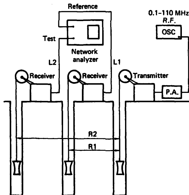
FIG. 7. Block diagram of the three-hole differential system to measure absolute transmission loss or phase change between boreholes.
