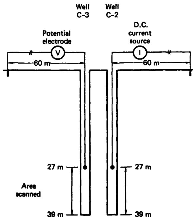
FIG. 2. Block diagram of cross-borehole resistivity system.
