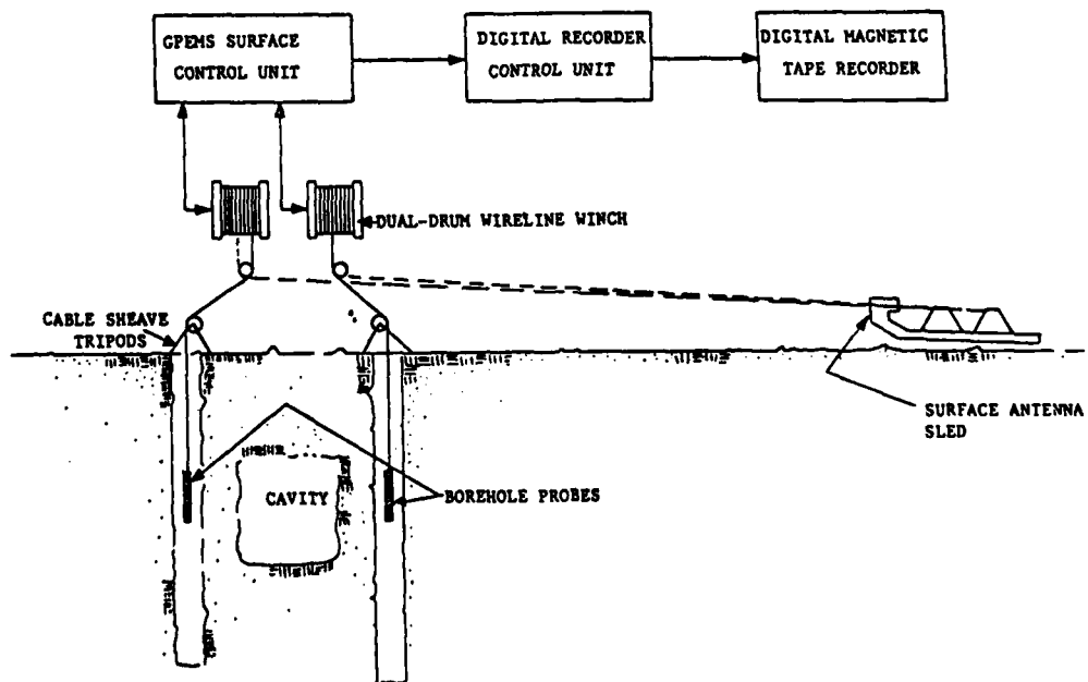
Figure 5. SwRI radar concept schematic
