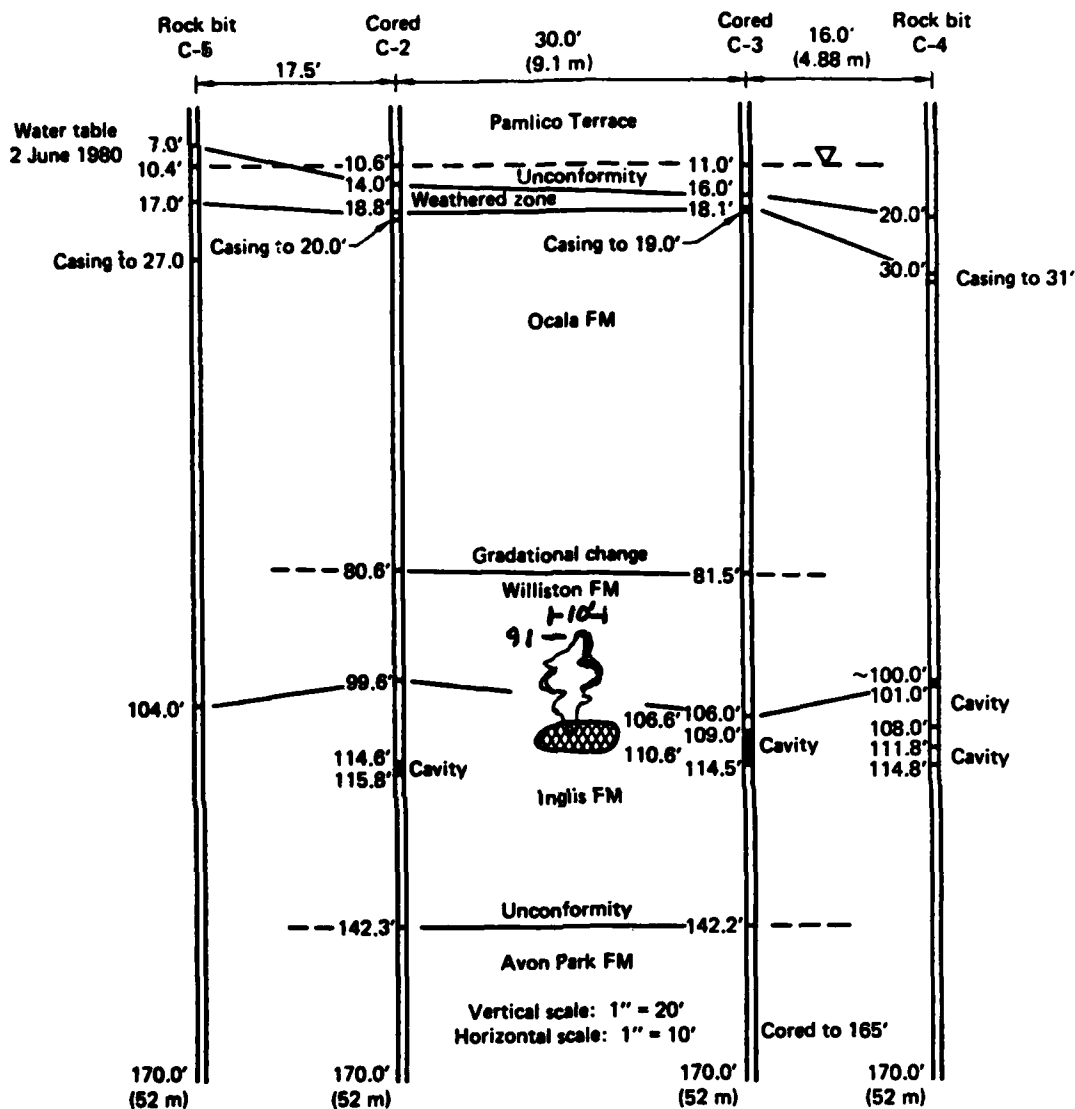
FIG. 4(b). Cross-sectional view of boreholes, Manatee Springs State Park, Florida.
