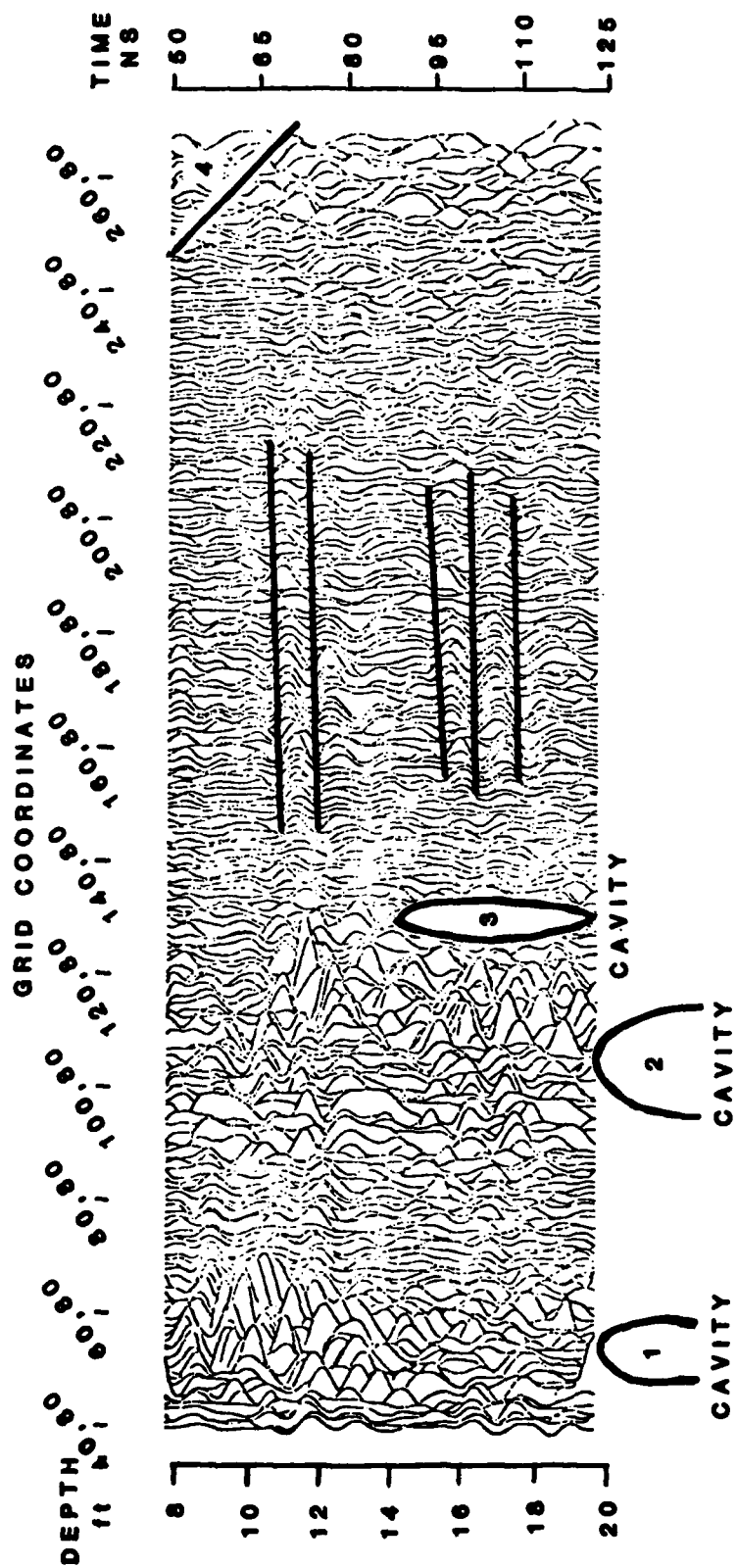
Figure 41. SwRI data obtained along north-south 80 grid line
