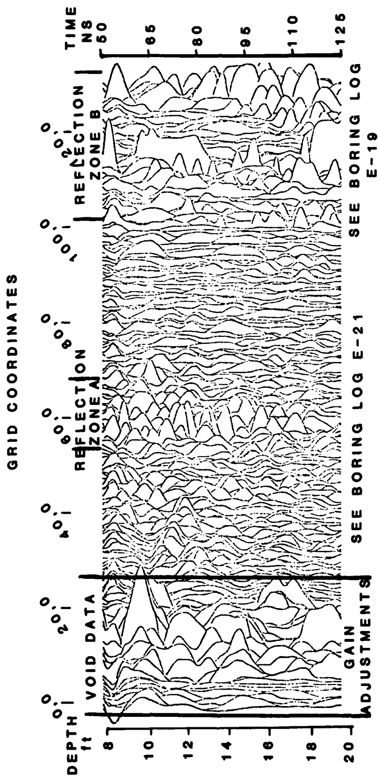
Figure 40. SwRI traverse line 11
