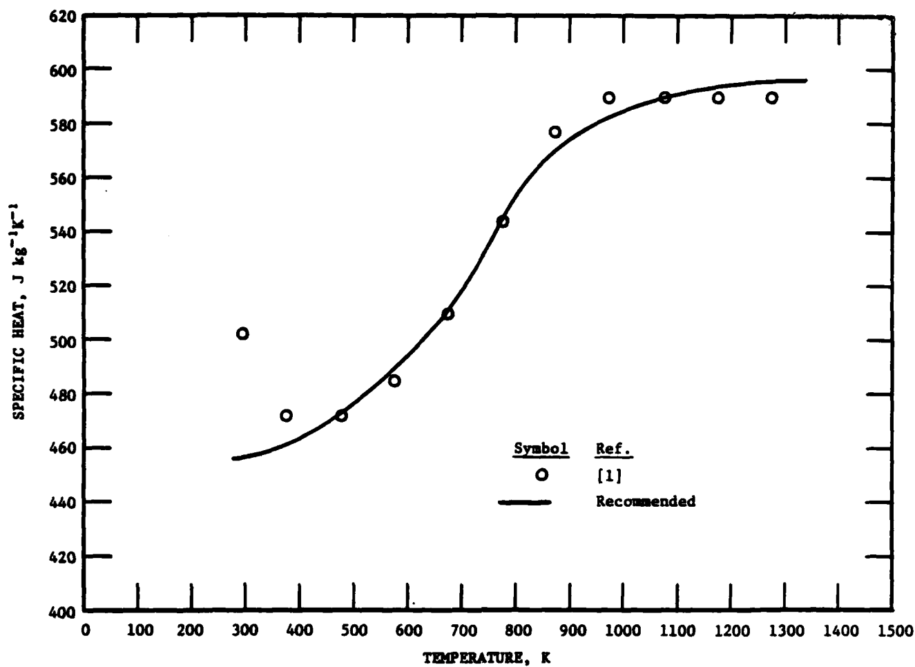
FIGURE 5.6. SPECIFIC HEAT OF X 8 CrNiMoNb 16 16 STAINLESS STEEL.
