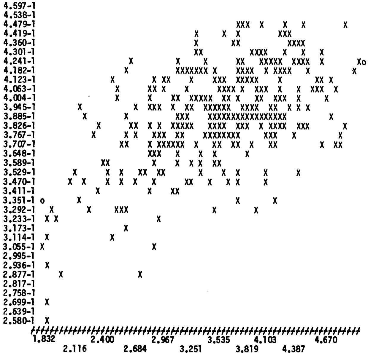
Figure A-1. Product-Moment Correlation Output
