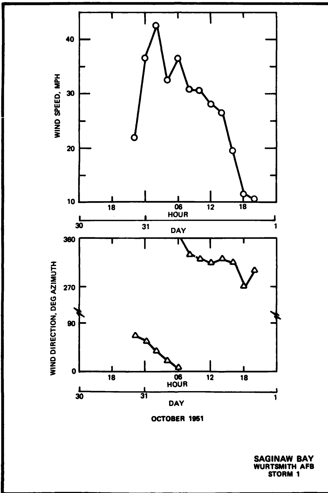
Figure A1. Wind data used for hindcast of storm of 30 October to 1 November 1951
