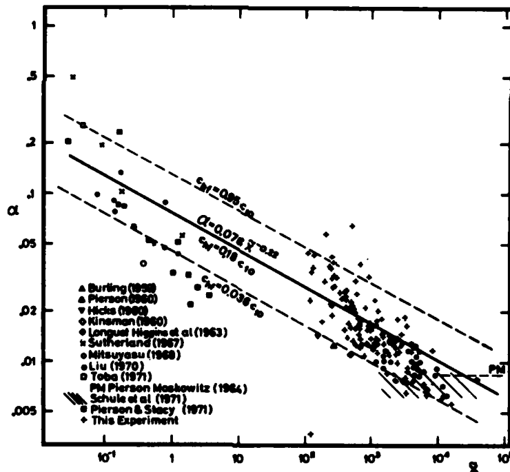
Phillips constant v. fetch scaled according to Kitaigorodskii. Small-fetch data are obtained from wind-wave tanks. (Capillary-wave data was excluded where possible.) Measurements by Sutherland (1967) and Toba (1971) were taken from W.I. Pierson and R.A. Stacy (1973)
