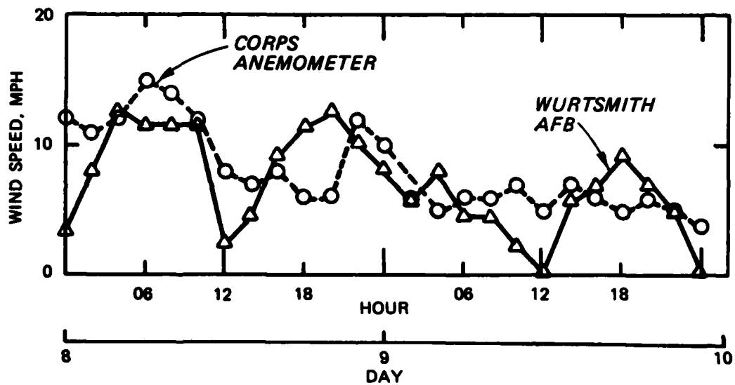
Figure 26. Comparison of wind data obtained at Wurtsmith AFB, Oscoda, Michigan, and CE Saginaw Projects Office, Essexville, Michigan, 8-10 October 1980
