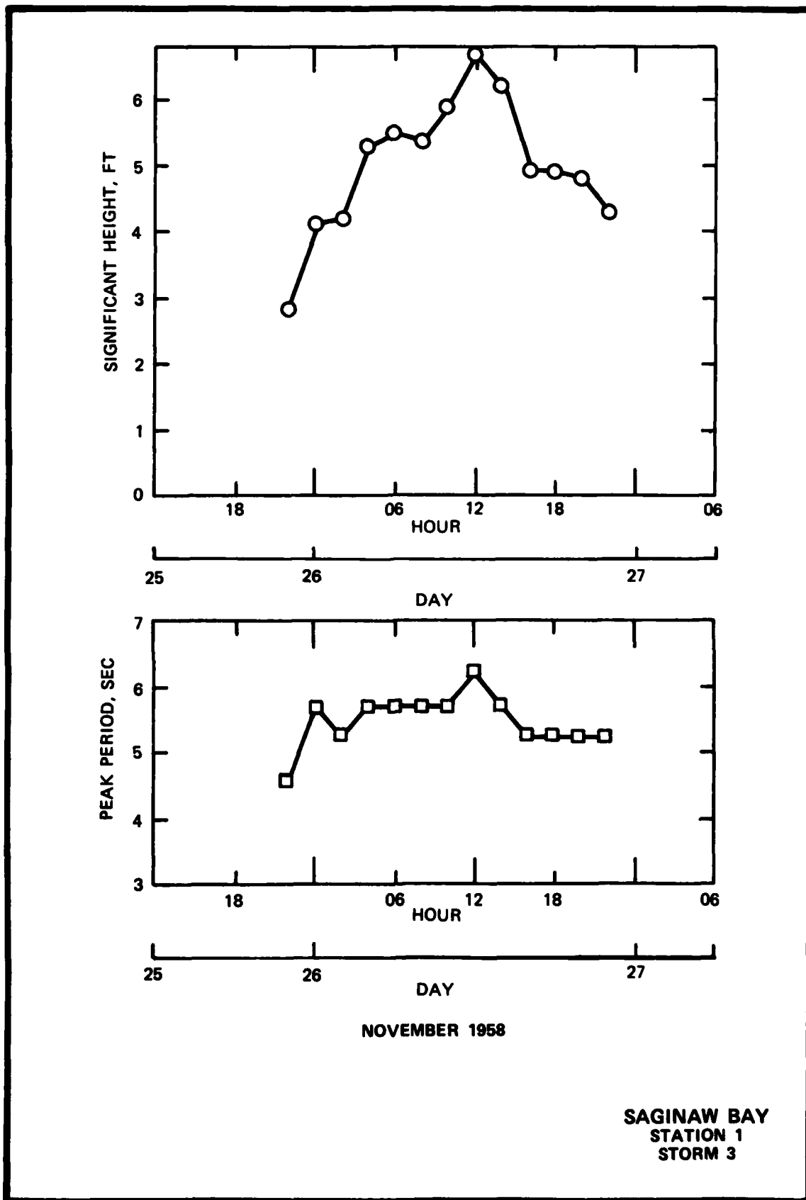
Figure A6. Hindcast significant wave height and peak wave period for storm of 25-27 November 1958
