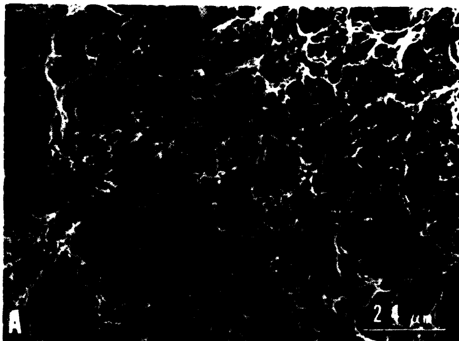
Figure 4. Scanning electron fractographs of a three-point bend specimen broken in the uncharged condition. (A) Low magnification fractograph showing the ductile rupture fracture mode.
