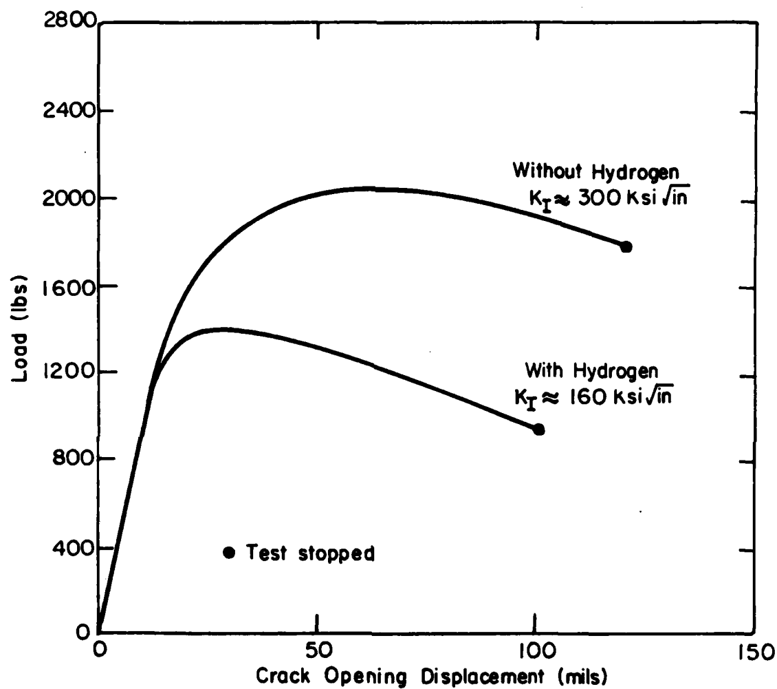
Figure 3. The load-displacement curves of three-point bend specimens of 5.5Ni steel tested before and after hydrogen charging.
