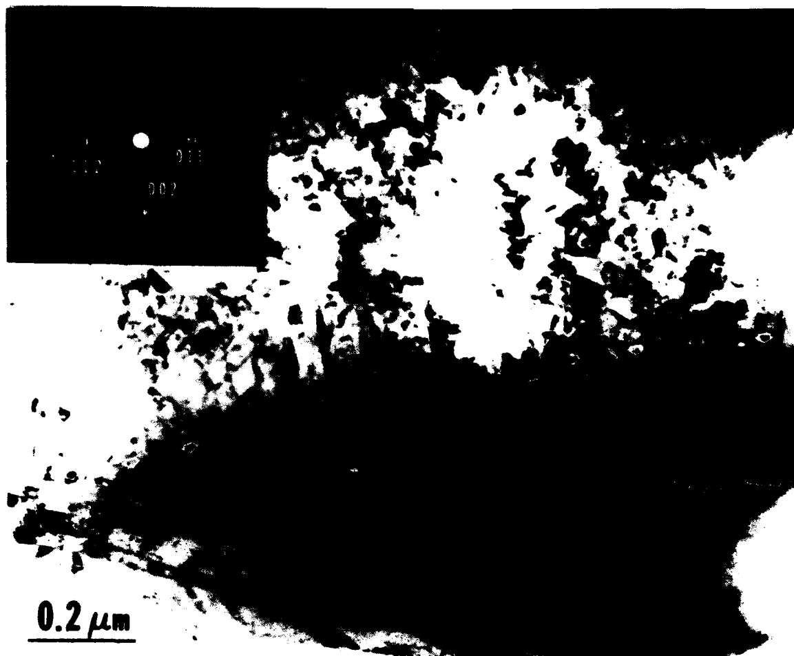
Figure 8. Transmission electron micrographs of the profile fractographic specimens showing the fracture surface and subsurface microcracks.
