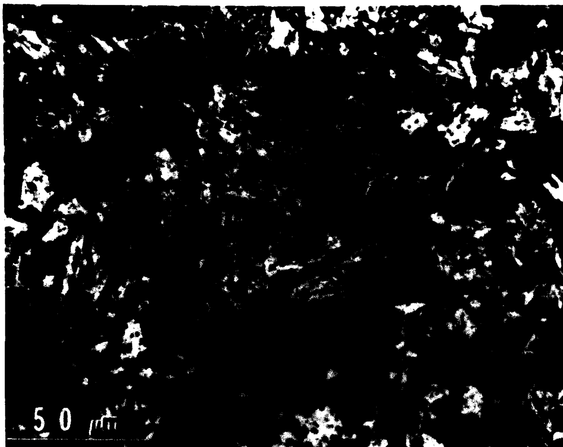
Figure 1. Optical micrograph of quenched and tempered 5.5Ni steel.
