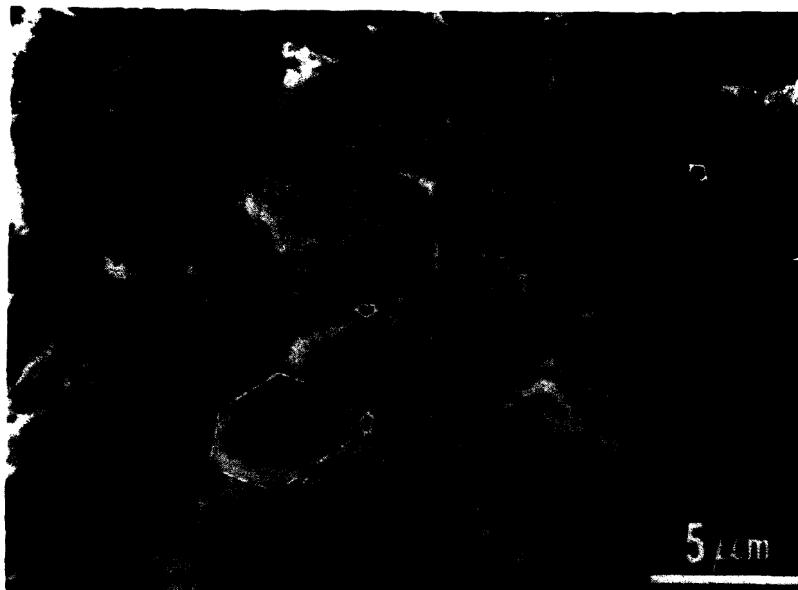
Figure 6. Scanning electron micrograph of the quasicleavage fracture surface after three-step etching with the reagent proposed in ref. 12. The outlined etch pit has a shape indicating a fracture plane near \{110\}
