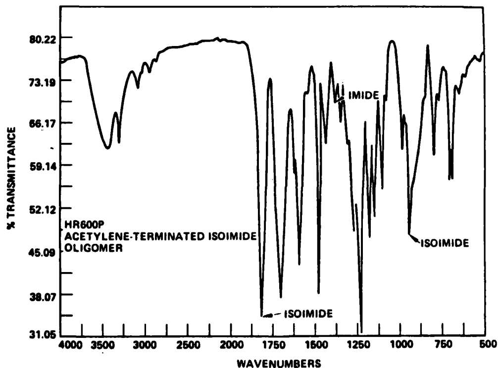
Figure 9. FTIR Spectrum of HR600P Acetylene-Terminated Isoimide Oligomer
