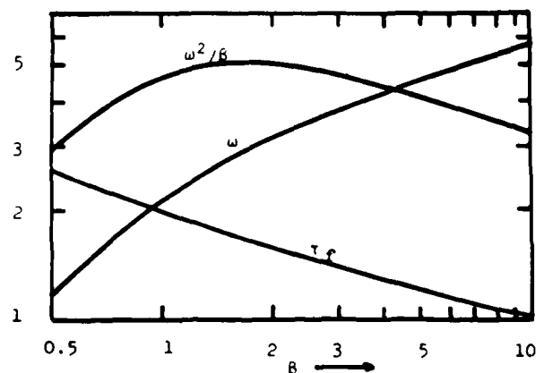
Figure 5. Results of zero-dimensional calculations.
