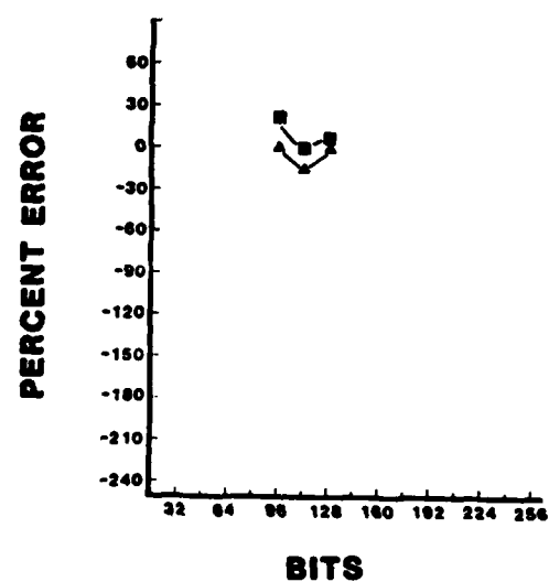
Figure 8. Upper percent error (■) and lower percent error (▲) as a function of bits for each of the red, green, and blue phosphors resulting from the model:
