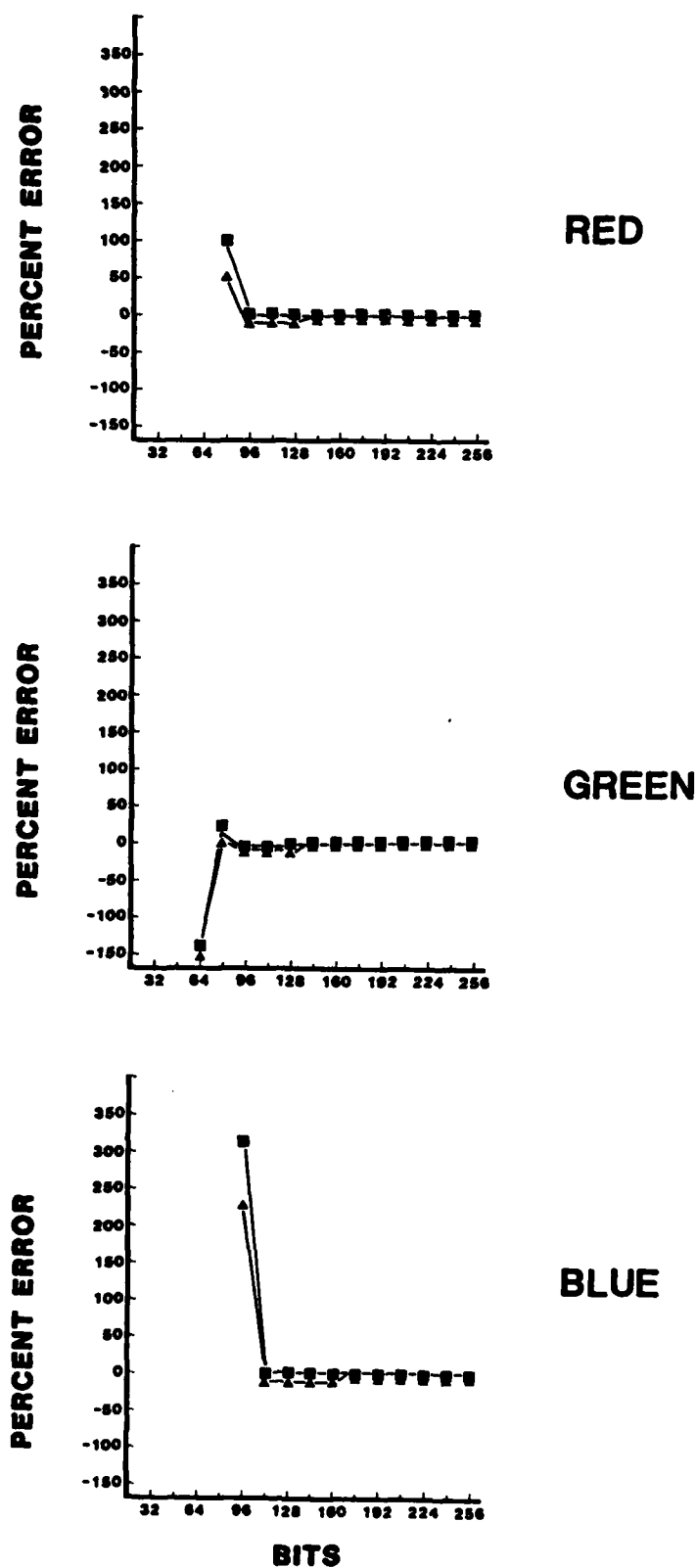
Figure 11. Upper percent error (■) and lower percent error (▲) as a function of bits for each of the red, green, and blue phosphors resulting from the model:
