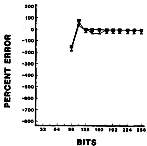
Figure 6. Upper percent error (■) and lower percent error (▲) as a function of bits for each of the red, green, and blue phosphors resulting from the model:
