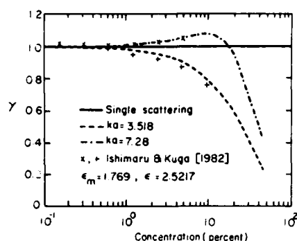
Fig. 6. Plot of \gamma = 2 \text{ Im } K / n_0 \sigma_t versus concentration where n_0 is the number density and \sigma_t is the extinction cross section of a single sphere with relevant ka .
