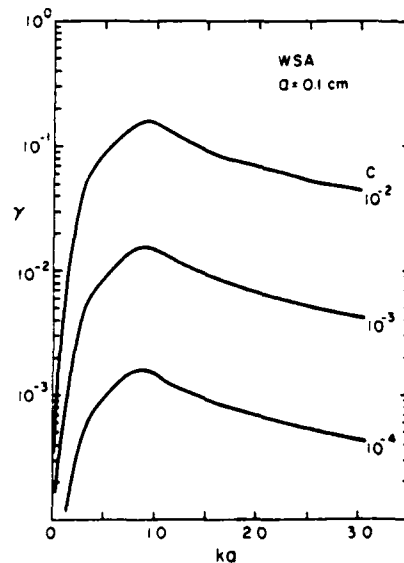
Fig. 3. The coherent attenuation constant \gamma versus ka for \epsilon_r = \epsilon_i(\lambda) using the WSA.
