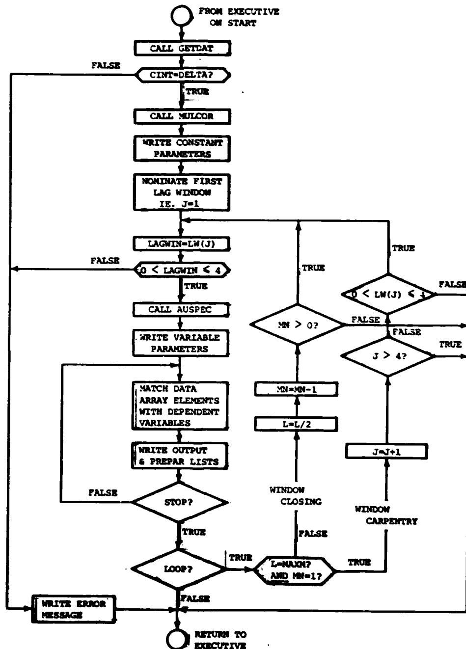
FIG. 2: Flowchart for SPECAN.CSL
