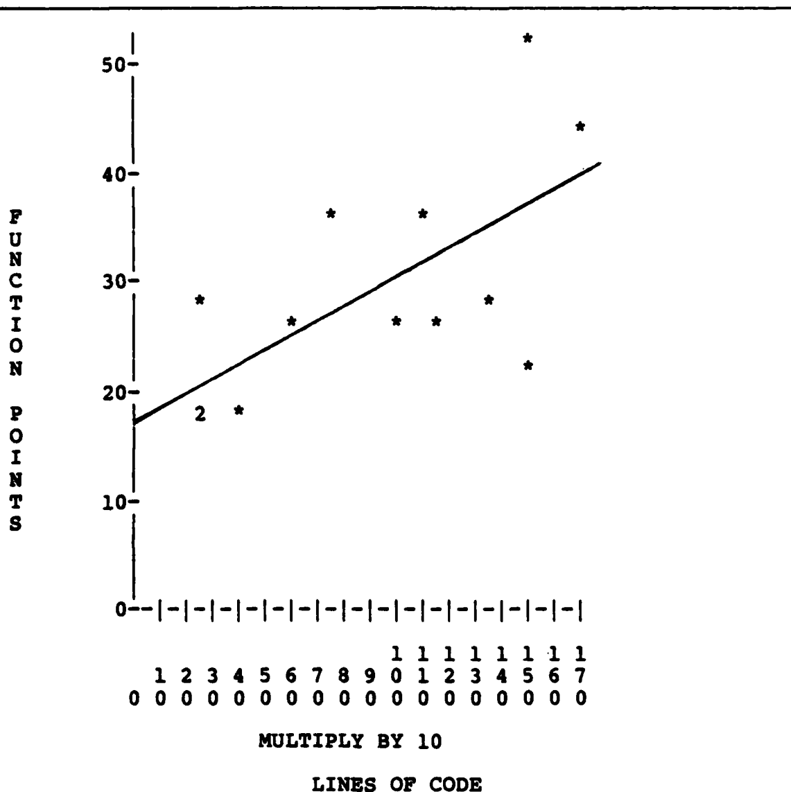
Figure 4.4 Function Points to Program Size Regression
