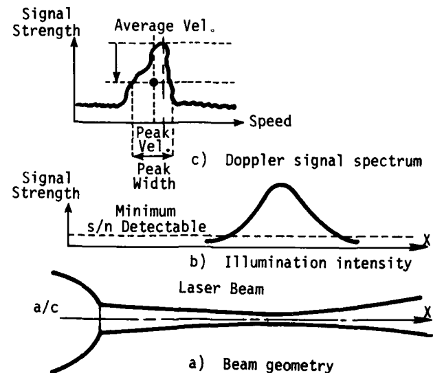
Figure 12. Principles of a CW Focussed Laser Anemometer
