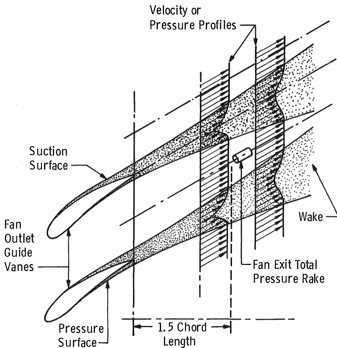
Fig.4.2.6 (Ref.4.2.7) Schematic of fan exit flow profile
