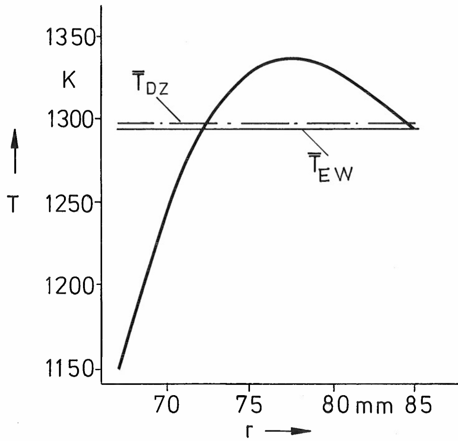
Fig.4.3.9 Section 2, static temperature
