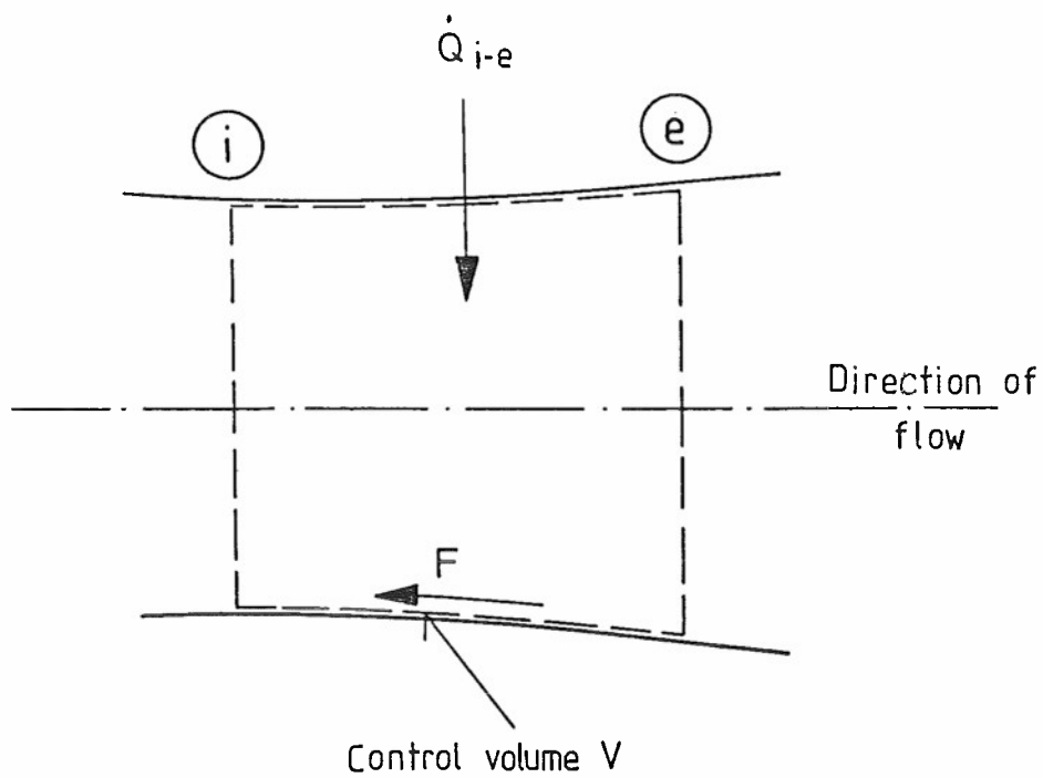
Fig.3.1.1 Swirl-free channel flow
