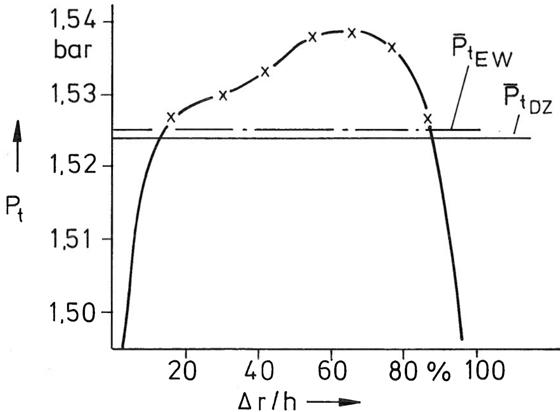
Fig.4.3.5 Section 4: Total pressure distribution
