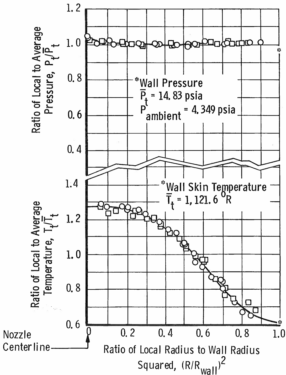
Fig.4.2.10 Measured nozzle total pressure and temperature profiles
