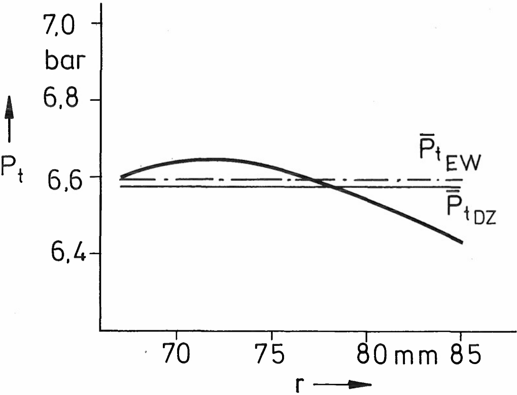
Fig.4.3.12 Section 3, total pressure
