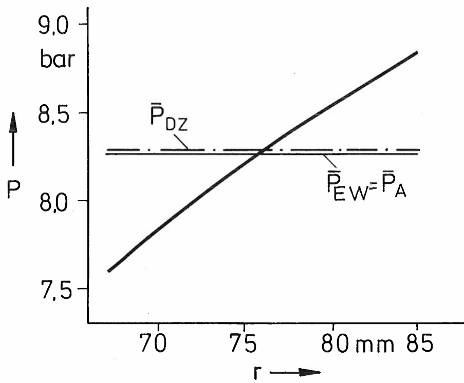
Fig.4.3.10 Section 2, static pressure
