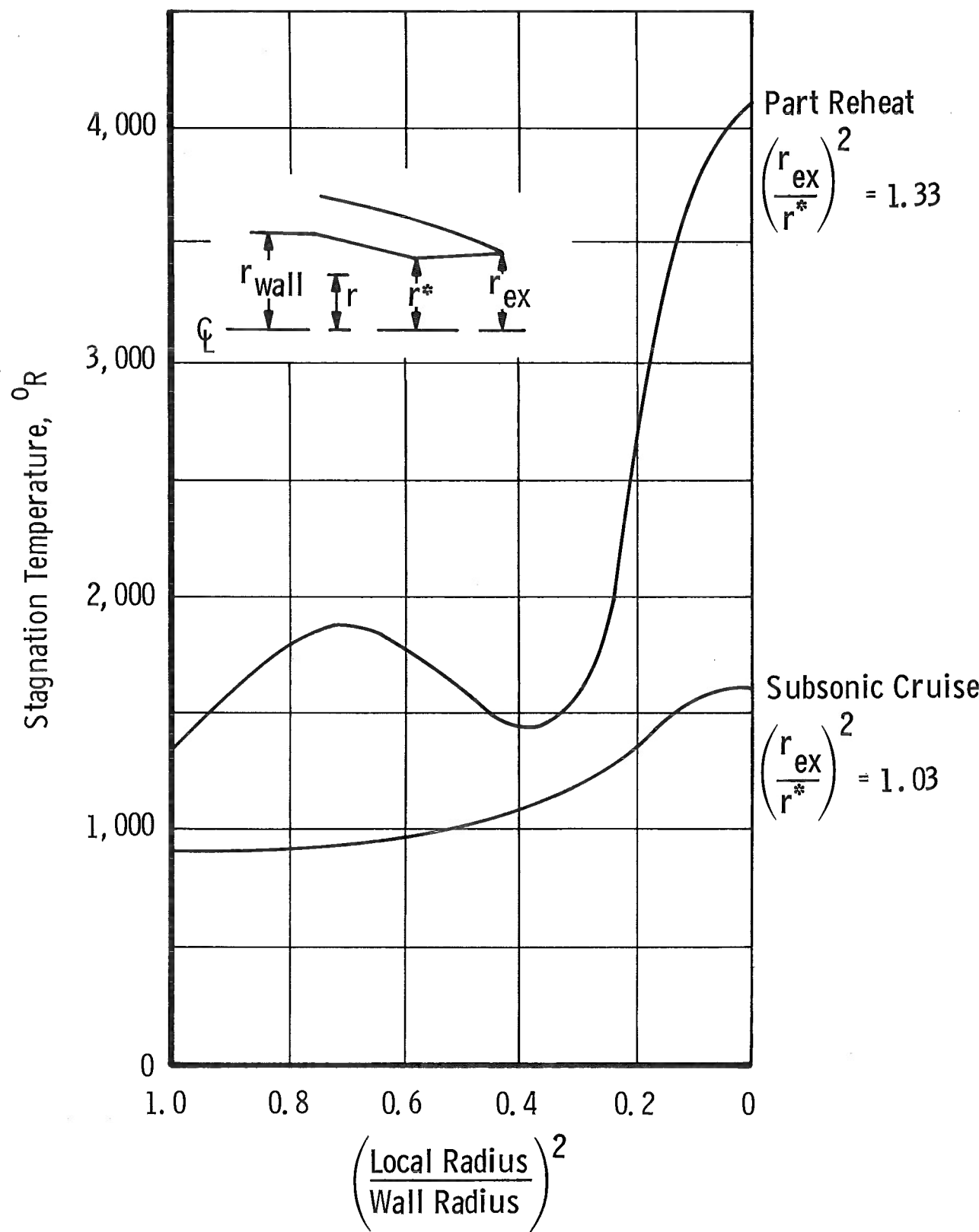
Fig.4.2.3 (Ref.4.2.3) Nozzle inlet temperature profiles
