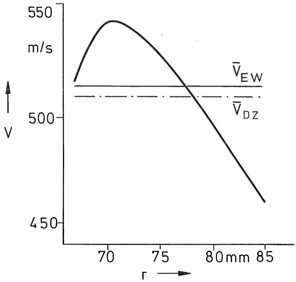
Fig.4.3.7 Section 2, velocity
