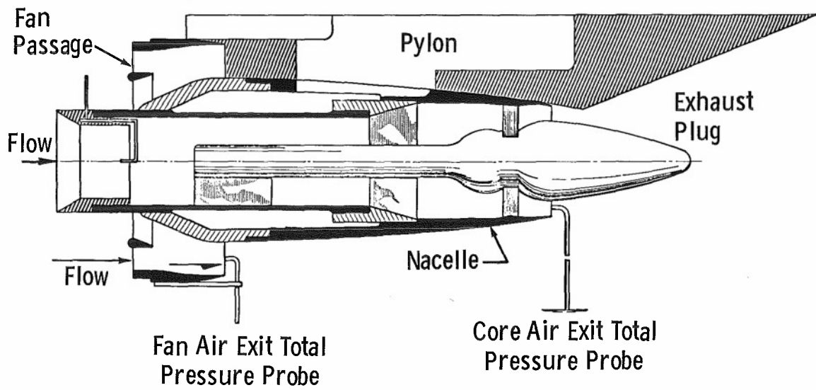
Fig.4.2.5 Schematic of dual stream turbofan engine
