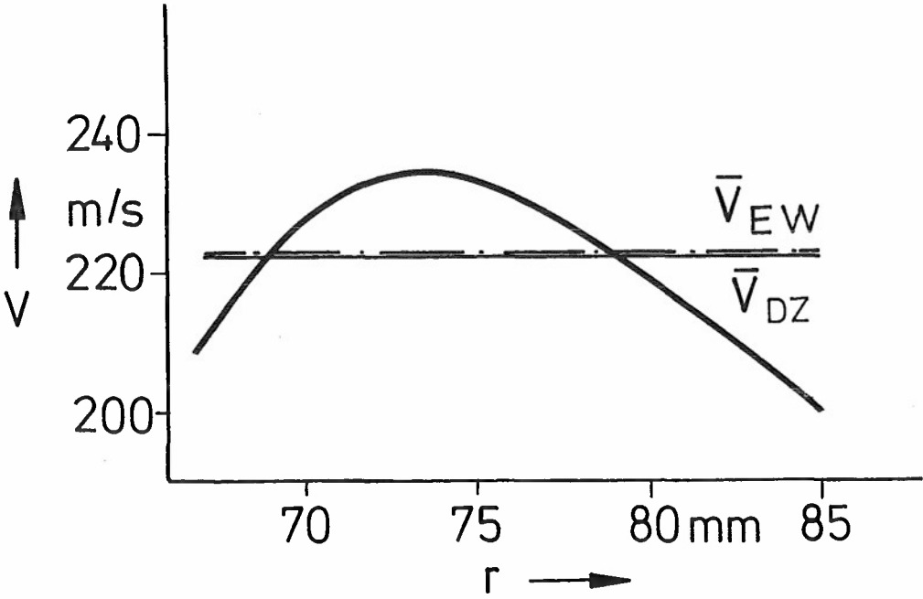
Fig.4.3.11 Section 3, velocity
