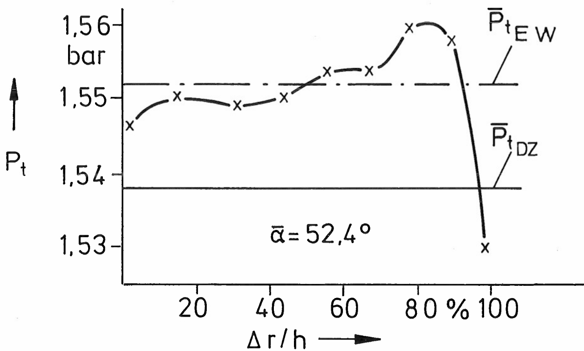
Fig.4.3.3 Section 2: Total pressure distribution
