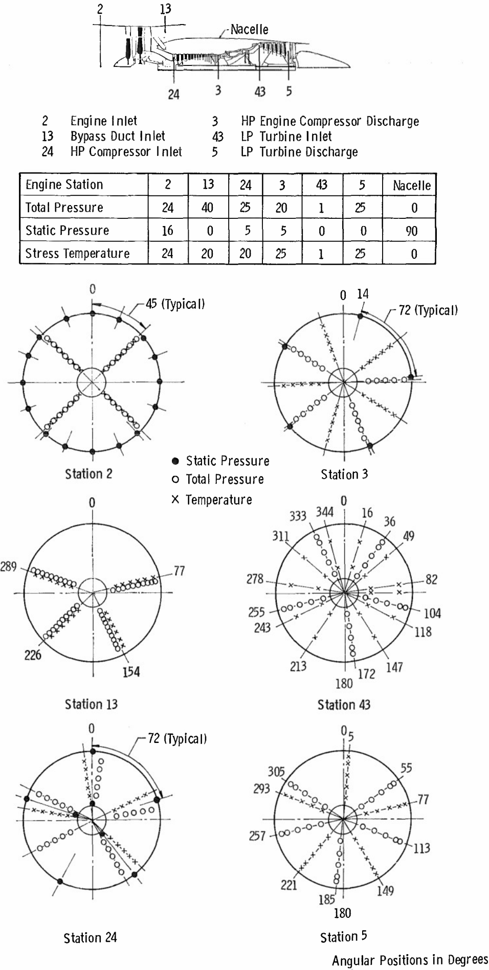
Fig.2.3 Dual-stream turbofan engine schematic and station designation
