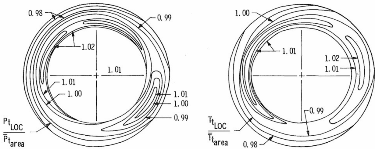
Fig.2.4 Representative high pressure compressor inlet total pressure and total temperature distributions (Ref.2.63)
