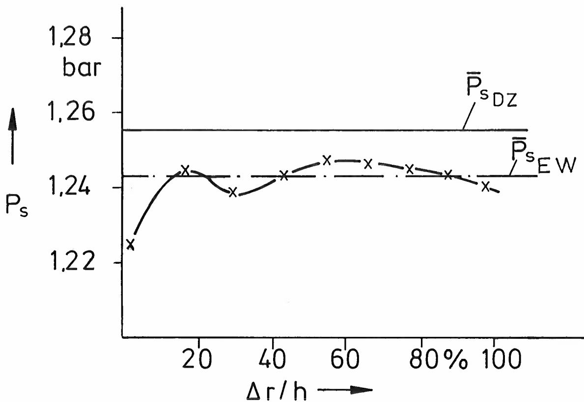
Fig.4.3.4 Section 4: Static pressure distribution
