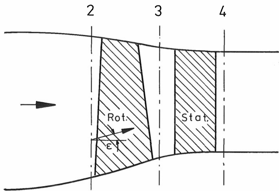
Fig.4.3.1 Geometry
