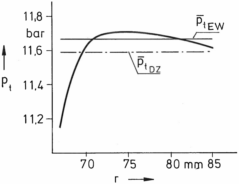
Fig.4.3.8 Section 2, total pressure
