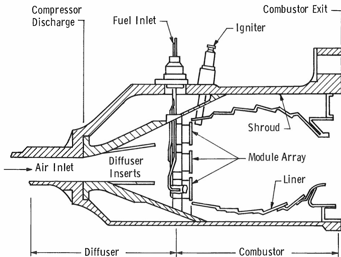
Fig.2.1 Annular swirl-can combustor
