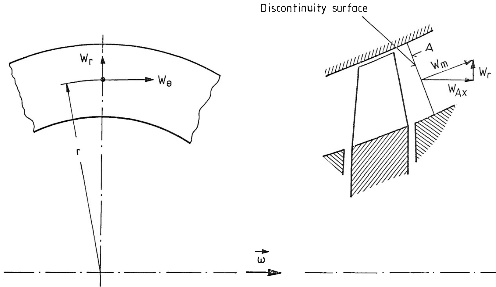
Fig.3.1.7 Discontinuity surface after a turbomachine rotor
