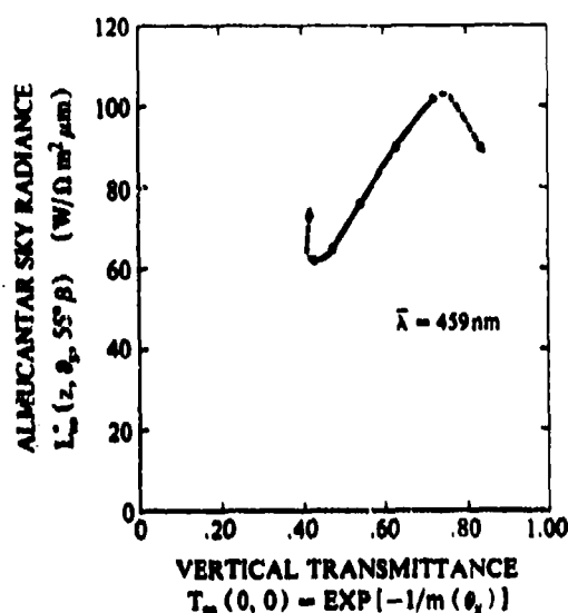
Fig. 3-4. Almucentar sky radiance at 55° vs vertical transmittance (Eq. 3.26) for 2 September 1964, filter 1 ( \lambda = 459 nm).
