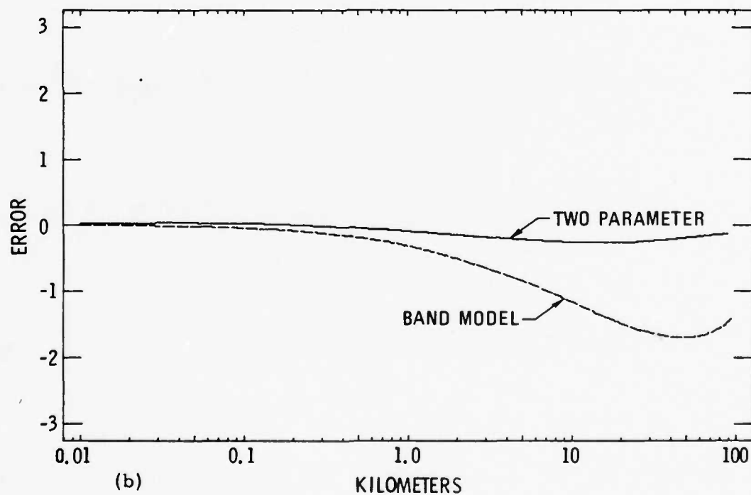
Fig. 19. Comparison of Line by Line ( \bar{T}_L ) and Alternate Two-Parameter Model ( \bar{T}_2 ) Transmittances for the 3040 \text{ cm}^{-1} Band. Error = \log_{10}(\bar{T}_2/\bar{T}_L) . The band model error is also shown for comparison.
