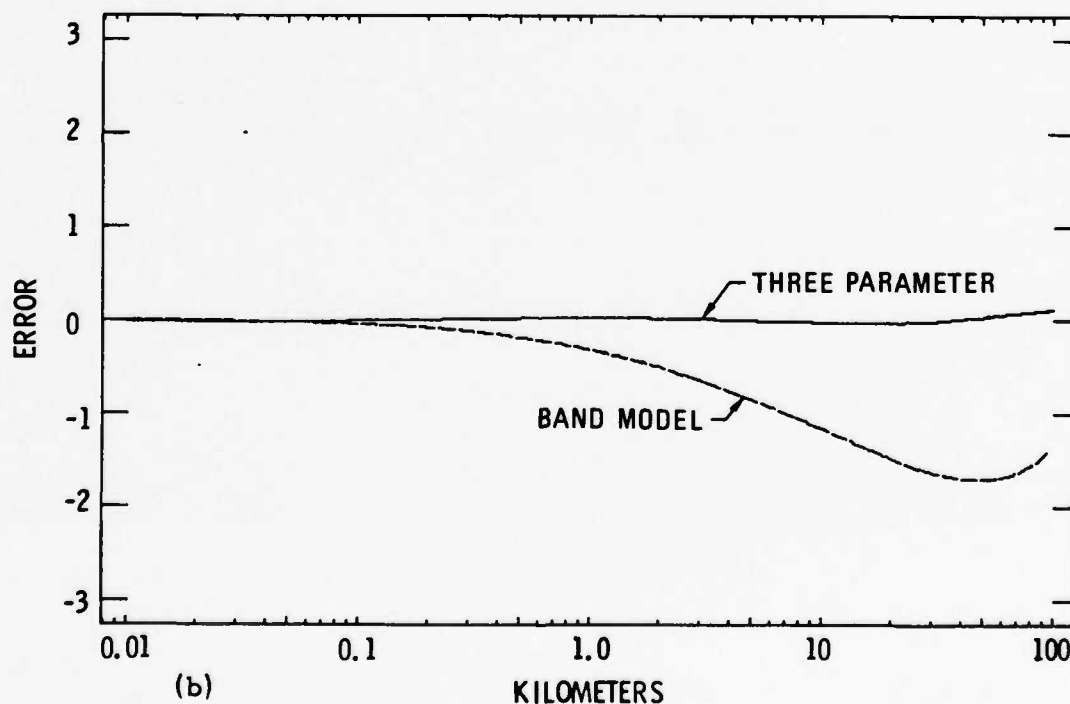
Fig. 23. Comparison of Line by Line ( \bar{T}_L ) and Three-Parameter Model ( \bar{T}_3 ) Transmittances for 3040 \text{ cm}^{-1} Band. Error = \text{Log}_{10}(\bar{T}_3/\bar{T}_L) . The band model error is also shown for comparison.
