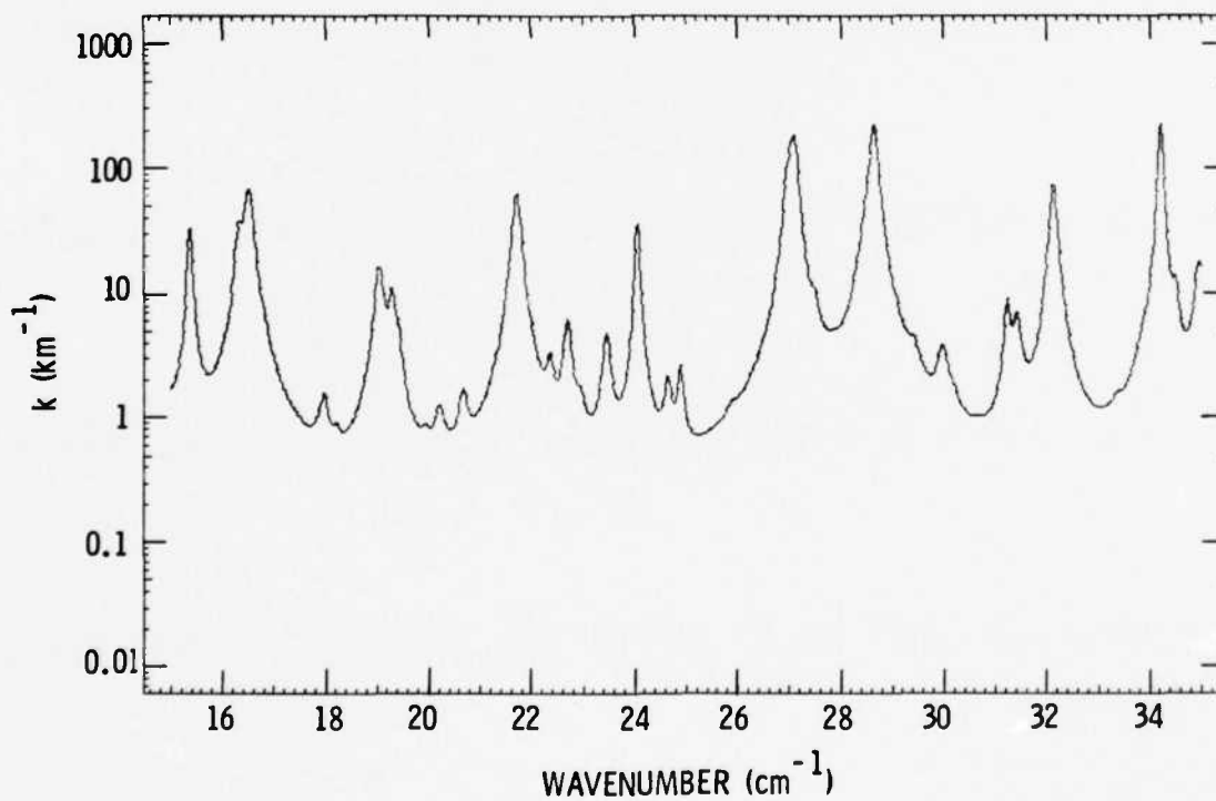
Fig. 12. Spectral Absorption Coefficient k(\nu) , Obtained from the Computer Generated Lines.
