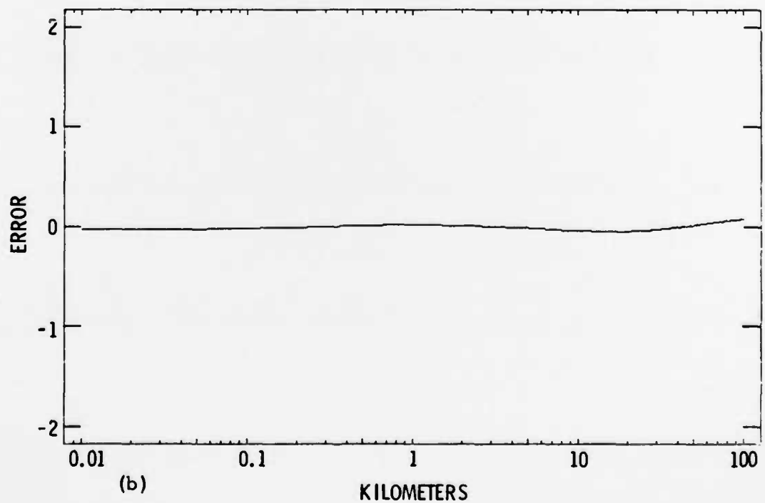
Fig. 27. Comparison of Line by Line ( \bar{T}_L ) and 50 Point Monte Carlo ( \bar{T}_{50} ) Transmittances for 3040 \text{ cm}^{-1} Band. Error = \log_{10}(\bar{T}_{50}/\bar{T}_L) .
