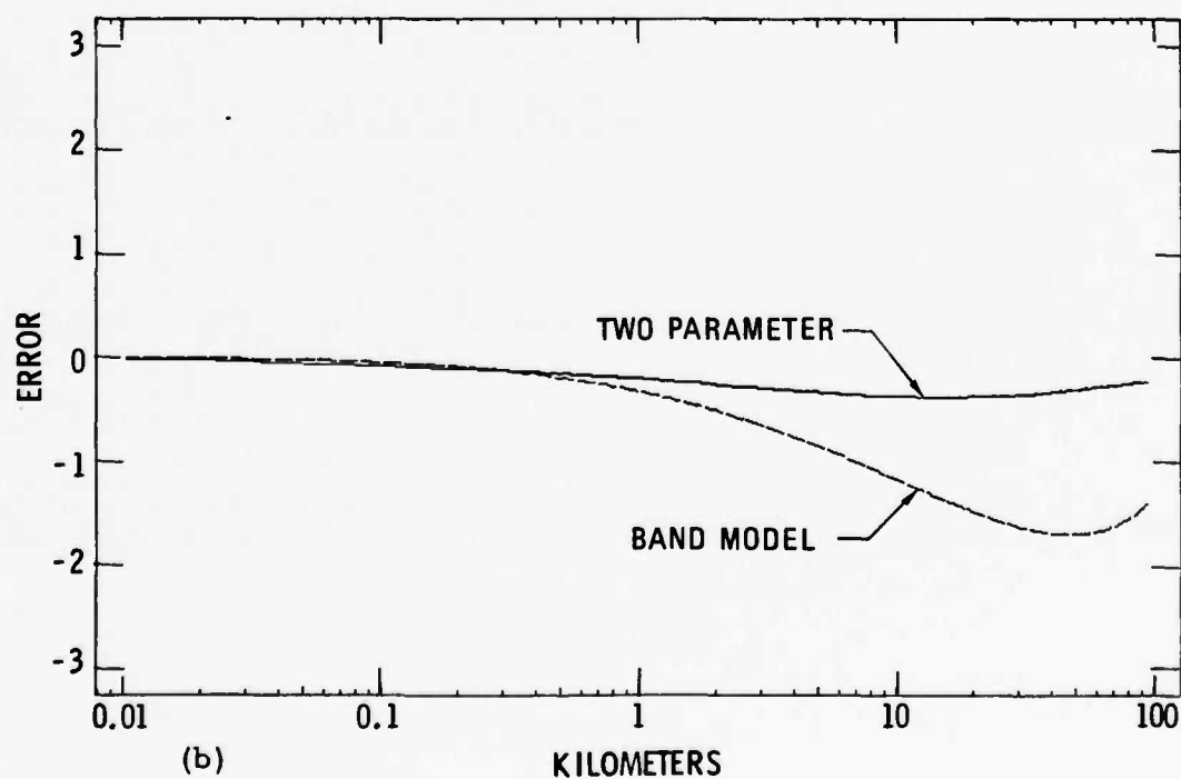
Fig. 16. Comparison of Line by Line ( \bar{T}_L ) and Two-Parameter Model ( \bar{T}_2 ) Transmittances for 3040 \text{ cm}^{-1} Band. Error = \log_{10}(\bar{T}_2/\bar{T}_L) . The band model error is also shown for comparison.
