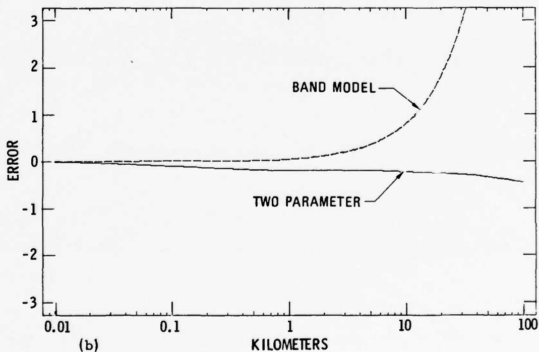
Fig. 17. Comparison of Line by Line ( \bar{T}_L ) and Two-Parameter Model ( \bar{T}_2 ) Transmittances for 3060\text{ cm}^{-1} Band. Error = \text{Log}_{10}(\bar{T}_2/\bar{T}_L) . The band model error is also shown for comparison.
