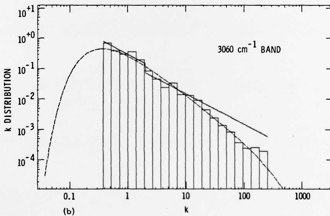
Fig. 25. k -Distribution Functions. Same as Fig. 24 except that the solid line is the three-parameter model.
