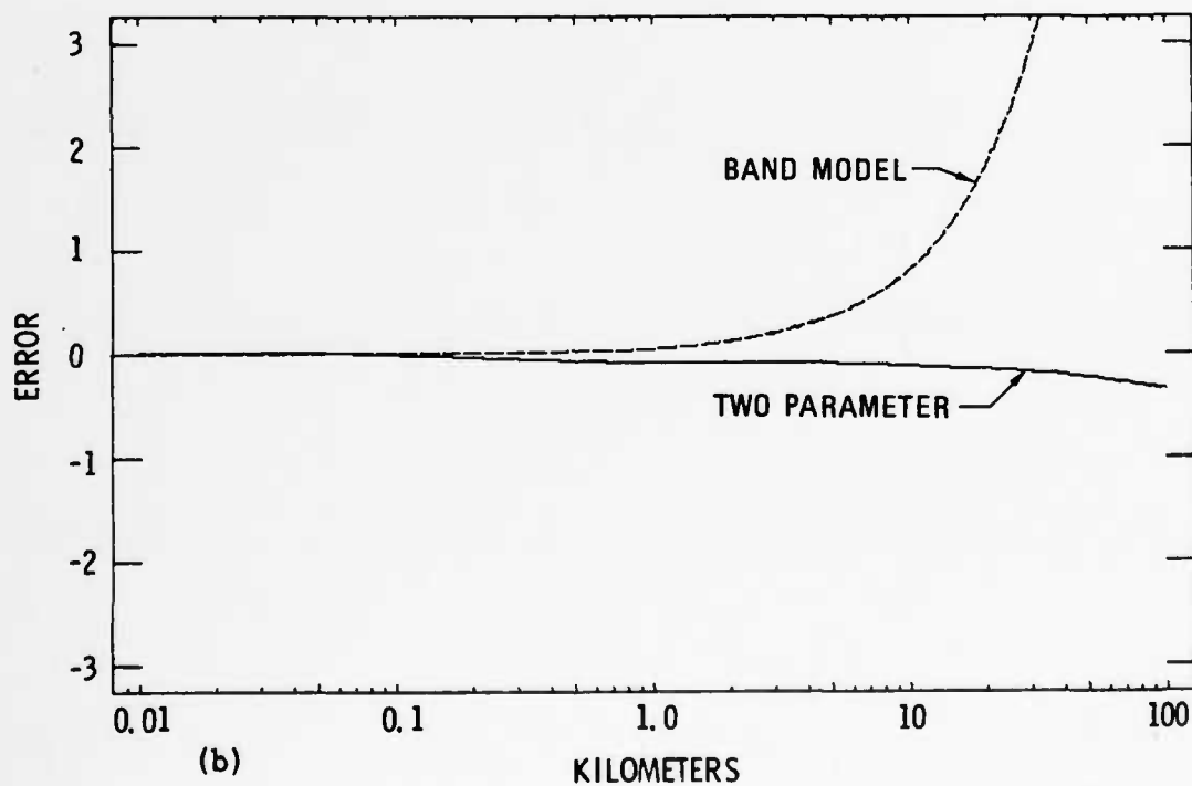
Fig. 20. Comparison of Line by Line ( \bar{T}_L ) and Alternate Two-Parameter Model ( \bar{T}_2 ) Transmittances for the 3060 \text{ cm}^{-1} Band. Error = \log_{10}(\bar{T}_2/\bar{T}_L) . Model error is also shown for comparison.
