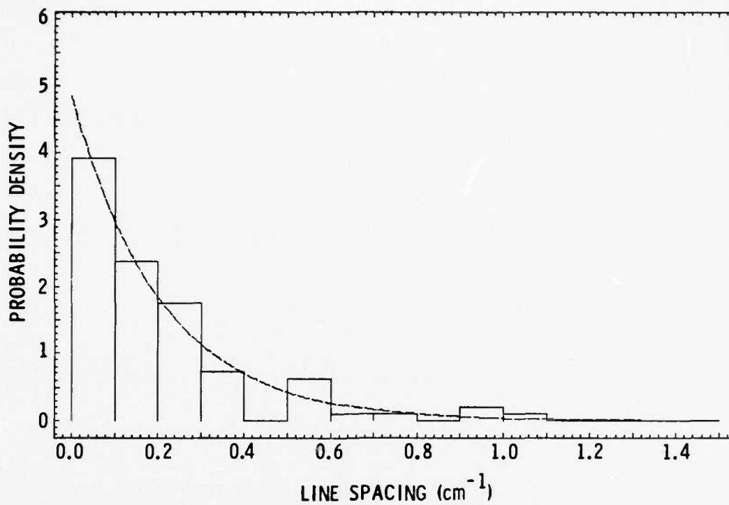
Fig. 11. Line Spacing Distribution for the Computer Generated Lines. Compare with Fig. 6.
