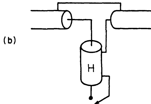
Fig. 7: The switch inductance (a) is modeled by a short line element (b).
