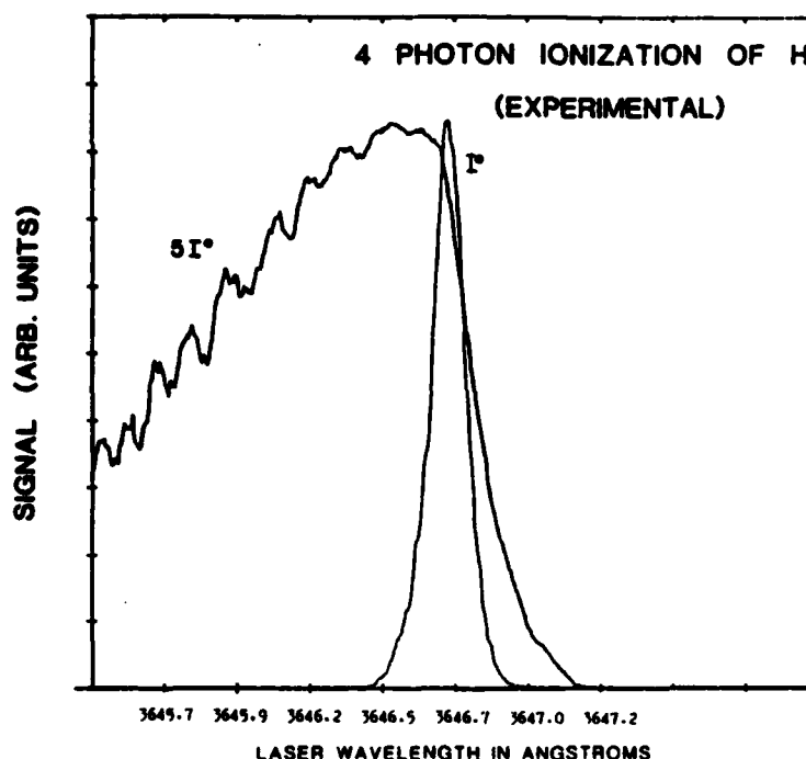
Figure 3-3: Ionization profiles produced by laser intensity 1^\circ and at five times that intensity 51^\circ . As the laser intensity is increased, the ionization profile becomes broad and asymmetric and is shifted to the blue of threshold.
