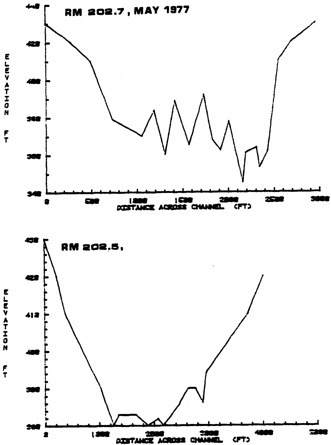
Figure 2.5. Cross section plots for Mississippi River between RM 196.8 and RM 202.7. The date of soundings is May 1977.
