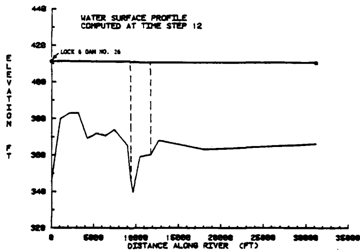
Figure 3.1. Water surface profiles, Mississippi River, RM 196.8 - 202.7.
