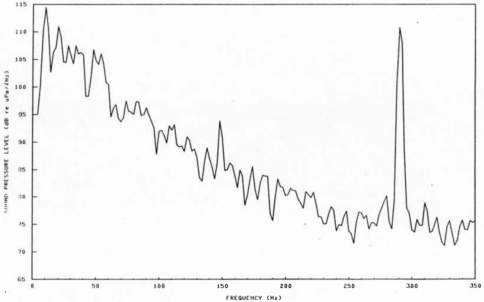
Spectrum of hydrophone #1 with the CW source 10 nmi west of SEACAL
