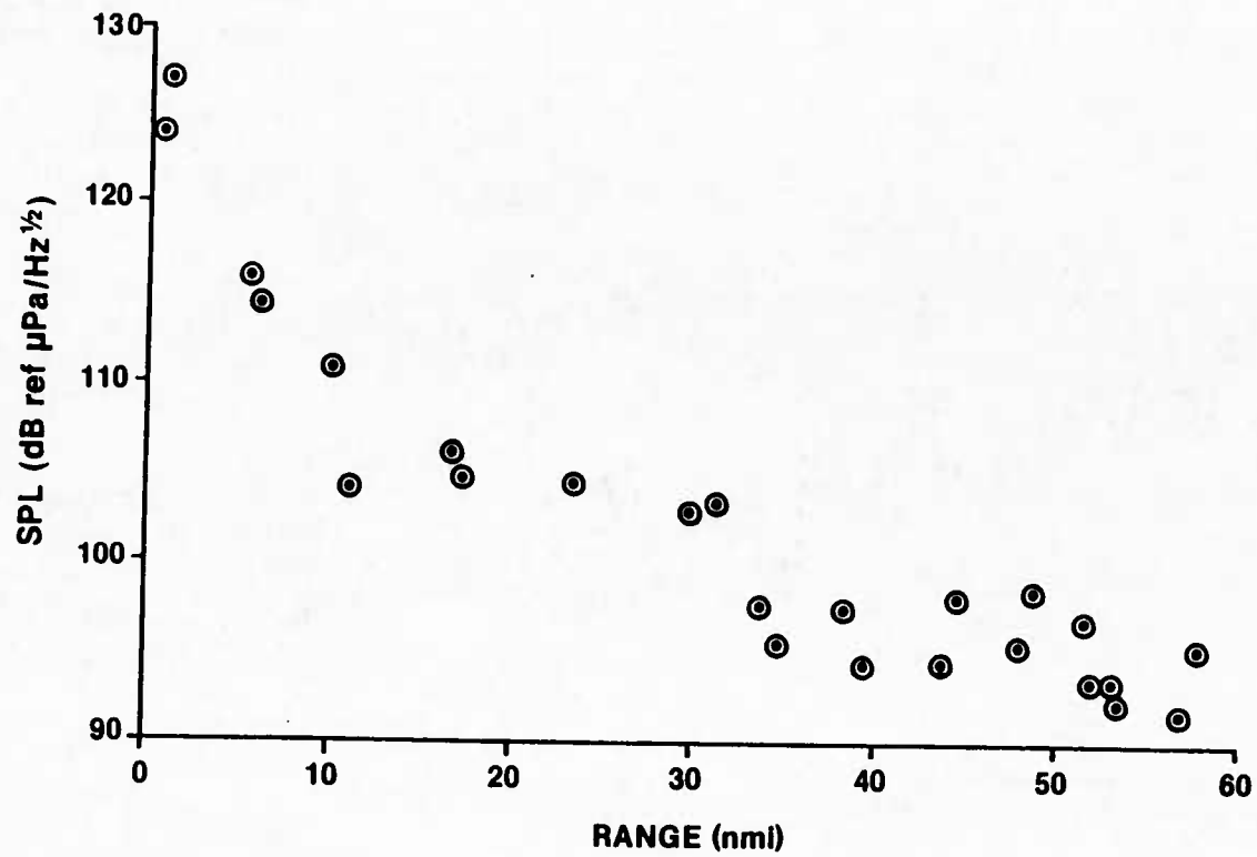
Received level of the 290 Hz tone as a function of range for hydrophone #1 during the 58 nmi CW tow
