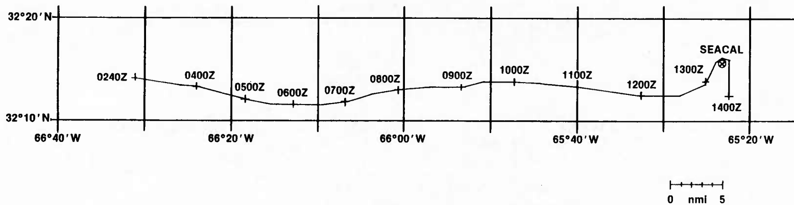
Ship Track of the CW tow commencing 58 nmi west of SEACAL for the period 0240 Z to 1400 Z on 09/10/83
