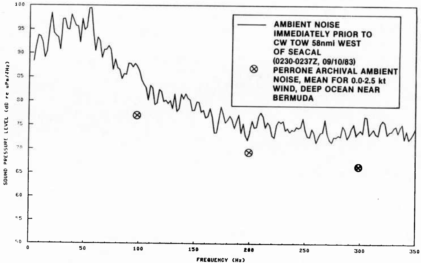
Ambient noise received on hydrophone #1 immediately prior to the CW tow 58 nmi west of SEACAL compared with archival measurements
