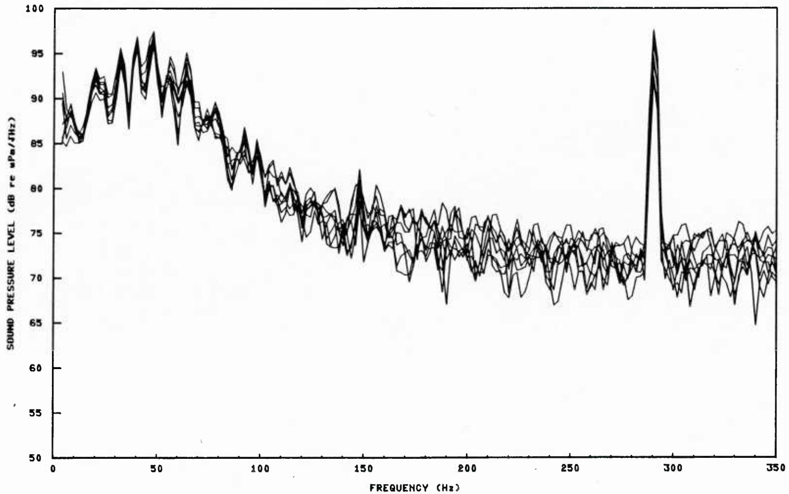
Spectra of the eight SEACAL hydrophones with the CW source 57 nmi west of SEACAL
