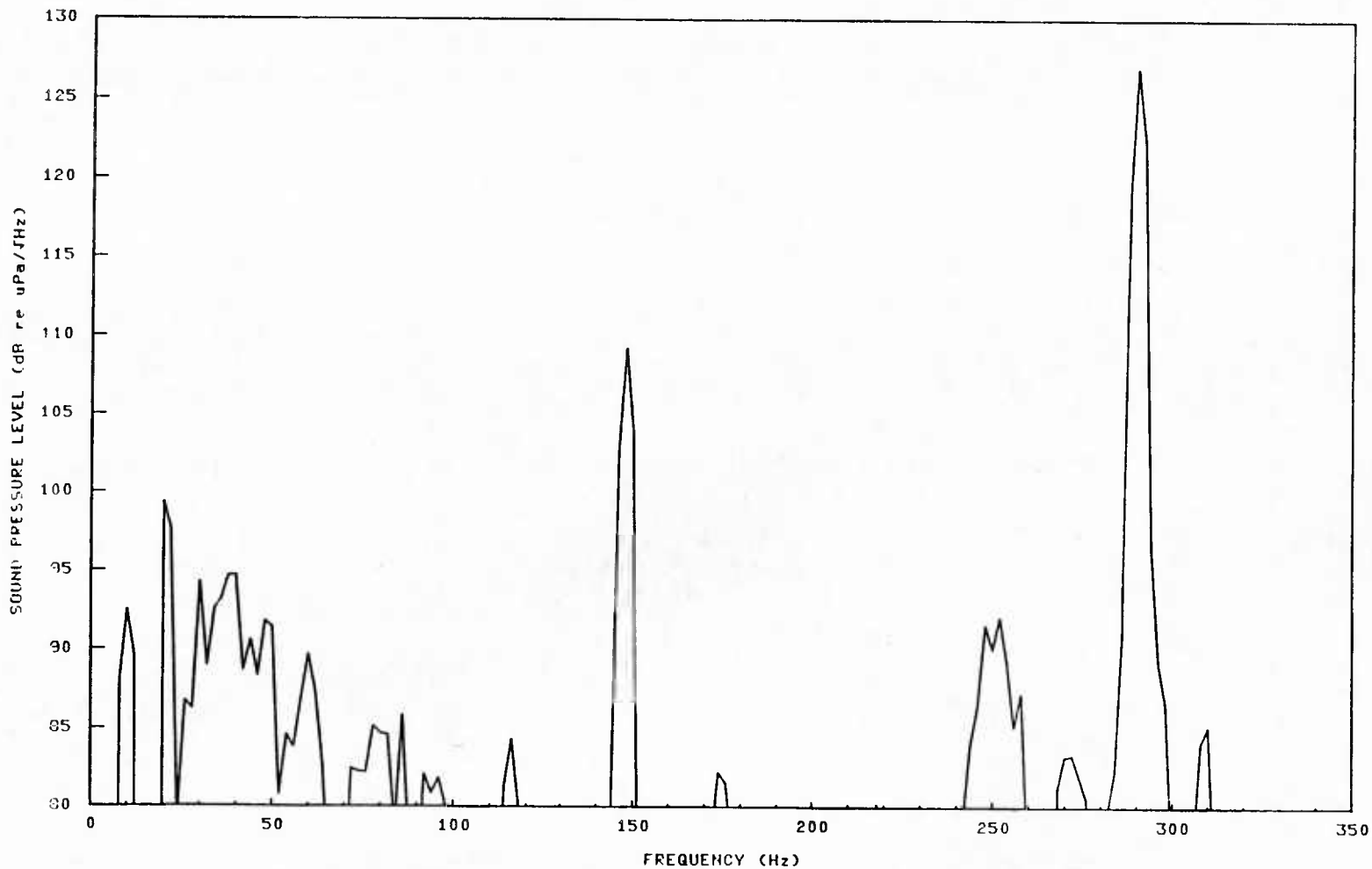
Spectrum of hydrophone #1 with the CW source 1 nmi southeast of SEACAL
