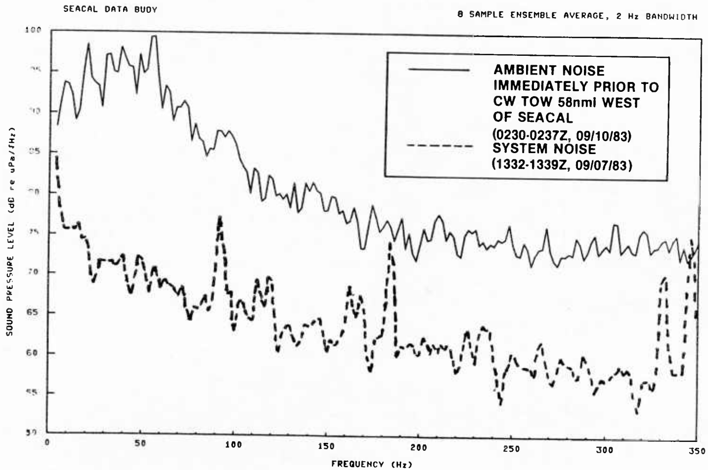
Ambient noise received on hydrophone #1 immediately prior to the CW tow 58 nmi west of SEACAL compared with system noise
