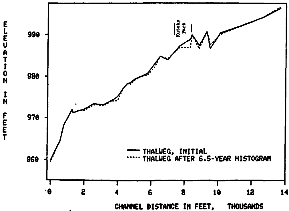
Figure 18. Cascade Creek, base test, existing conditions
