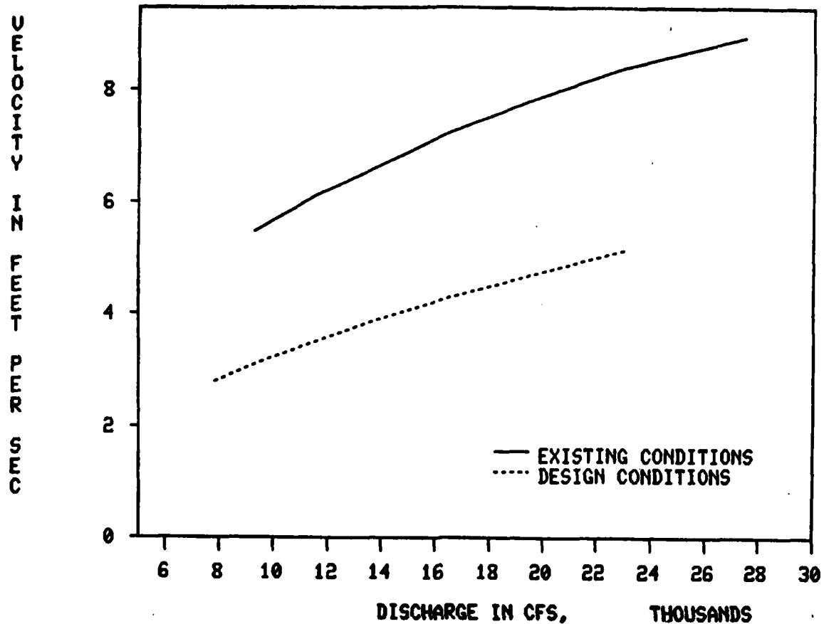
Figure 22. Section 29, comparison of existing and design water velocities
