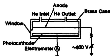
Fig. 1 The ex situ EXAFS detector and sample chamber.
