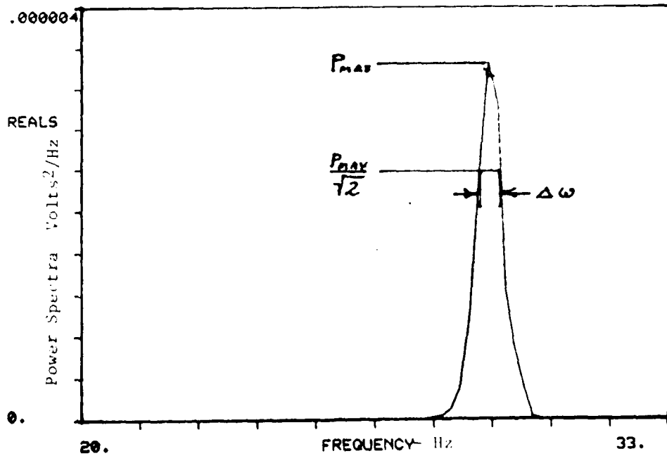
Figure 18. Damping Coefficient by Half-Power Point
