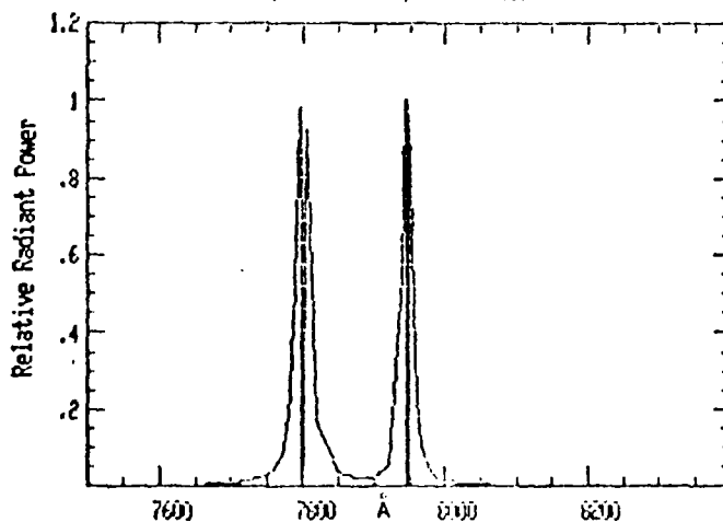
Figure A-58 Rubidium at 6 Torr 35% Mg, 60% RbNO 3 , 5% Binder
