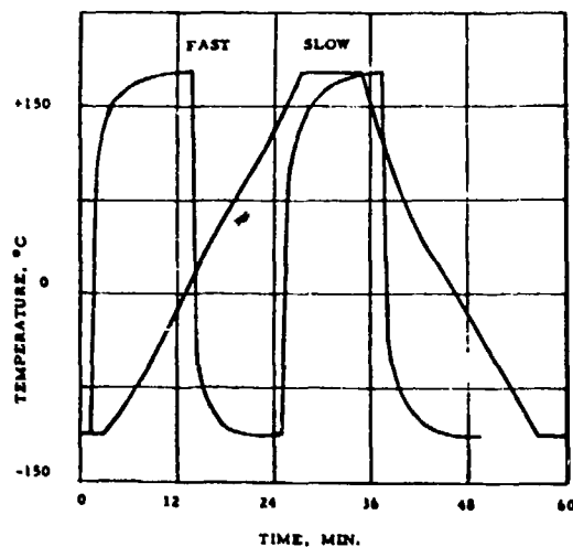
FIG. 4: SCHEMATIC OF THERMAL CYCLES FOR TEMPERATURE CYCLING SYSTEMS[268]
