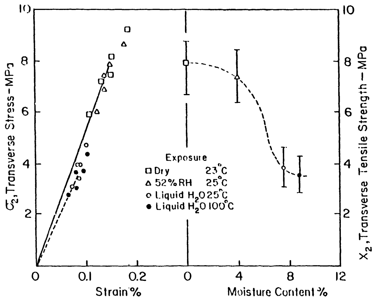
FIG. 16: TRANSVERSE TENSILE BEHAVIOR OF K-49 EPOXY AT DIFFERENT ENVIRONMENTAL CONDITIONS. LEFT, AVERAGE STRESS-STRAIN RESPONSES AND FAILURE POINTS; RIGHT, TRANSVERSE TENSILE STRENGTH AS A FUNCTION OF MOISTURE CONTENTS ( \text{MPa} \times 0.145 = \text{Ksi} ) [322]
