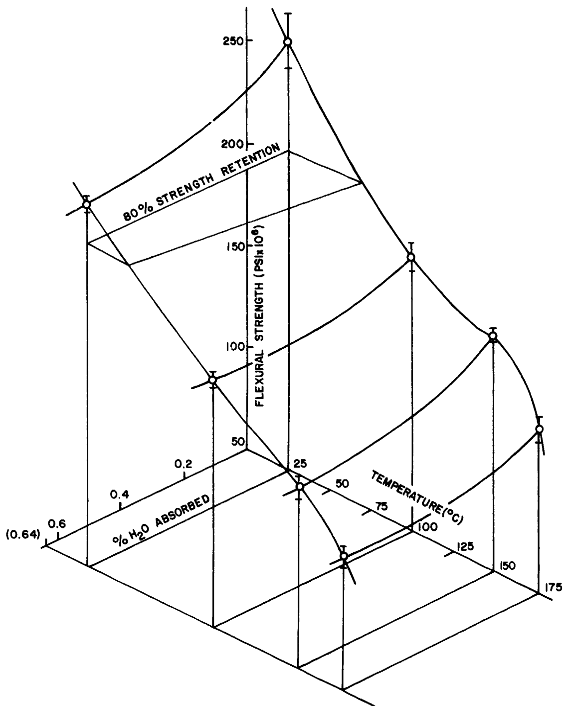
FIG. 11: FLEXURAL STRENGTH OF UNIDIRECTIONAL CARBON FIBER COMPOSITES (NARMCO 5208/T300) AS A FUNCTION OF TEMPERATURE AND PERCENT MOISTURE ABSORBED [23]
