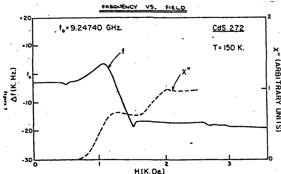
Fig. 6. The frequency and loss of the microwave cavity containing a specimen of pressure quenched CdS as a function of magnetic field.
