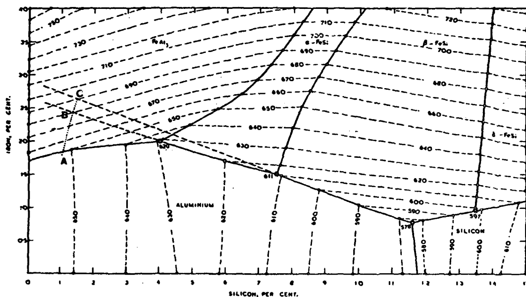
Fig. 9. Liquidus surface of the Al-rich corner of the Al-Fe-Si system [31]. If the phase Fe 3 Al does not form, the eutectic valley, L → α-Al + α-FeSi, extends toward B and the Al-Fe binary. In the absence of both Fe 3 Al and α-FeSi, the eutectic valley L → α-Al + β-FeSi extends toward C and the Al-Fe binary. The solidification path for an alloy of composi- tion A during formation of primary α-Al would follow the line AB before the formation of α-FeSi in the first case and AC before the formation of β-FeSi in the second case.
