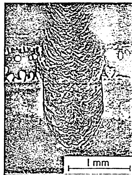
Fig. 8. Electron beam scan at 0.2 m/s across eutectic band.
