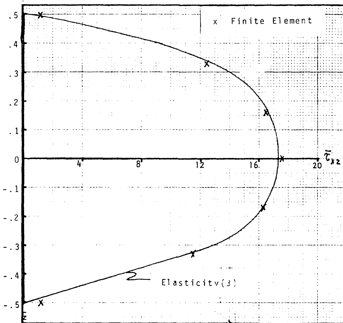
FIGURE 4.11: Semi-infinite Plate Case 1: \bar{\tau}_{xz} vs. \bar{z} , S=4 .
