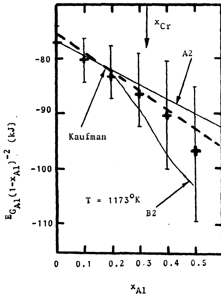
Figure 4b. The Partial Excess Gibbs Free Energy of Aluminum in bcc iron-aluminum alloys at 1173°K divided by the atomic fraction of iron squared shown as a function of the aluminum concentration. The heavy line is due to Kaufman and Nesor (Reference 9) while the crosses (and error bars) are from Hultgren (Reference 10). The remaining curves refer to the present analysis.
