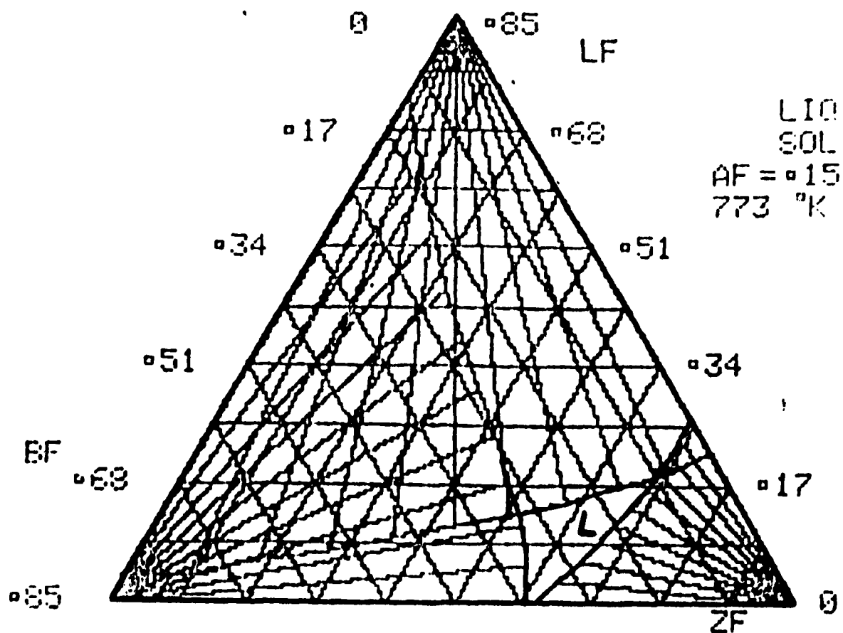
Figure 5 Calculated Solid-Liquid Equilibria in LF-ZF-BF with AF=0.09 (above) AF=0.15 (below)
