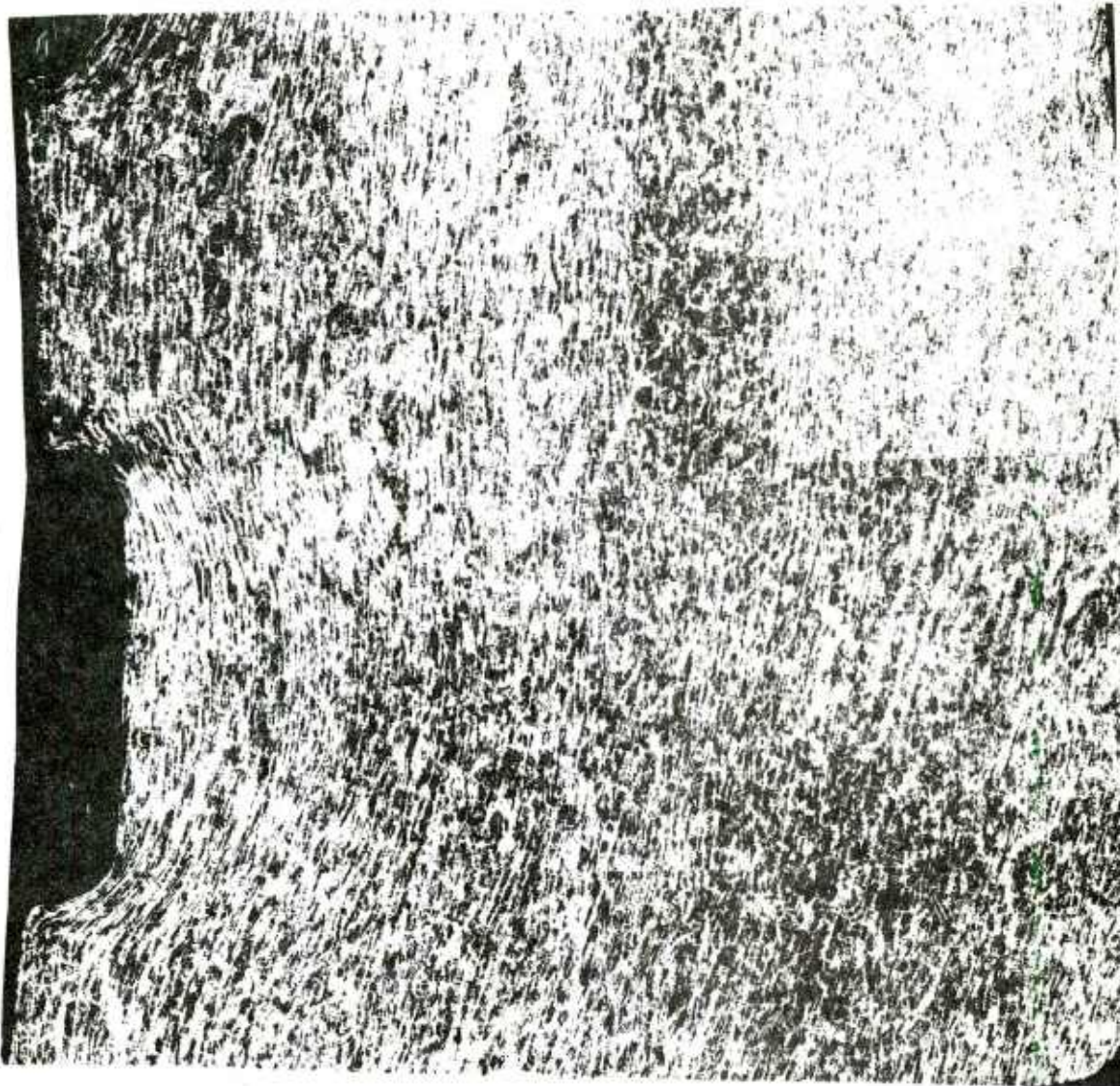
FORGED RIFLING IN 105mm GUN TUBE TRANSVERSE, 20 X
