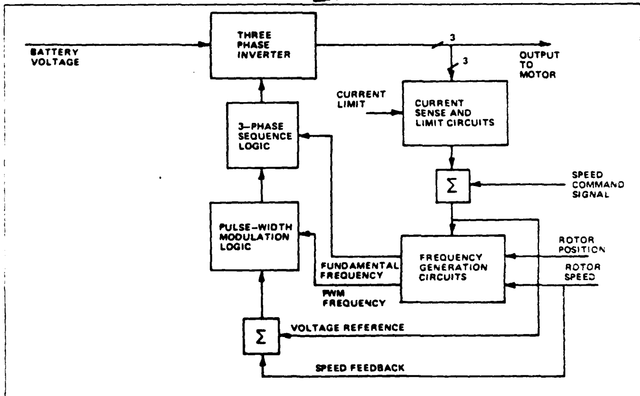
Figure B 4, Controller Block Diagram
