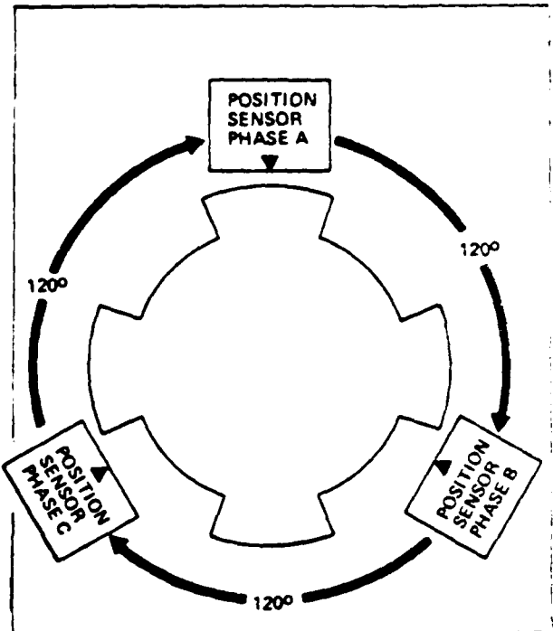
Figure B 3 Rotor Position Sensing
