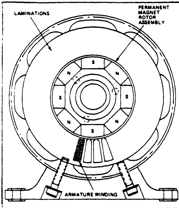
Figure B 2, End View of Motor
