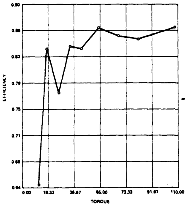
Figure 4 - Sundstrand Motor Test
