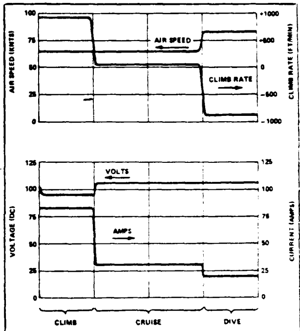
Figure 5 - Performance Parameters
