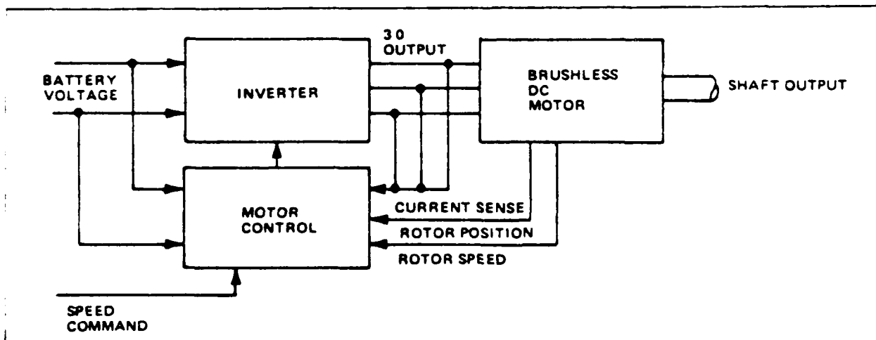
Figure 6-10. Motor and Control
