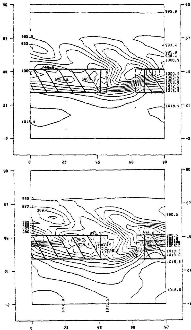
Figure 31. Sea-Level Pressure, 90 and 102 h, Exp. 5.
