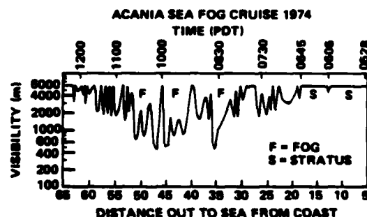
FIG. 6. Visibility data as a function of distance obtained while cruising crosswind through a series of fog patches, 23 August 1974.
