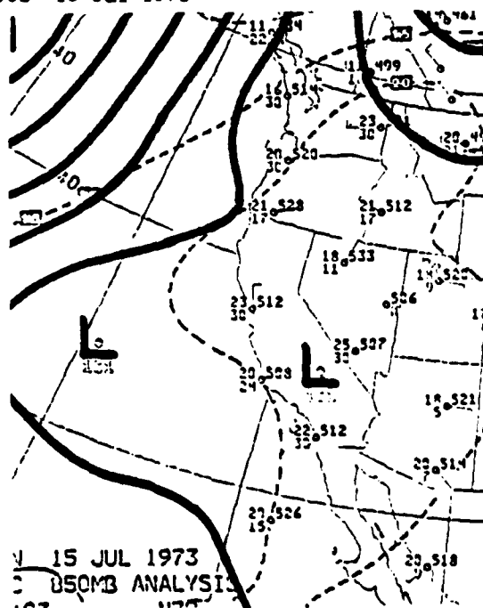
850 mb Analysis 12Z 15 Jul 1973
