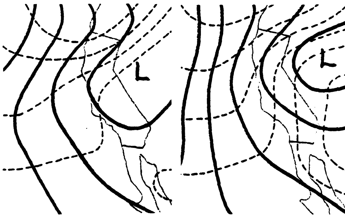
850 mb Analysis 12Z 22 May 1978
