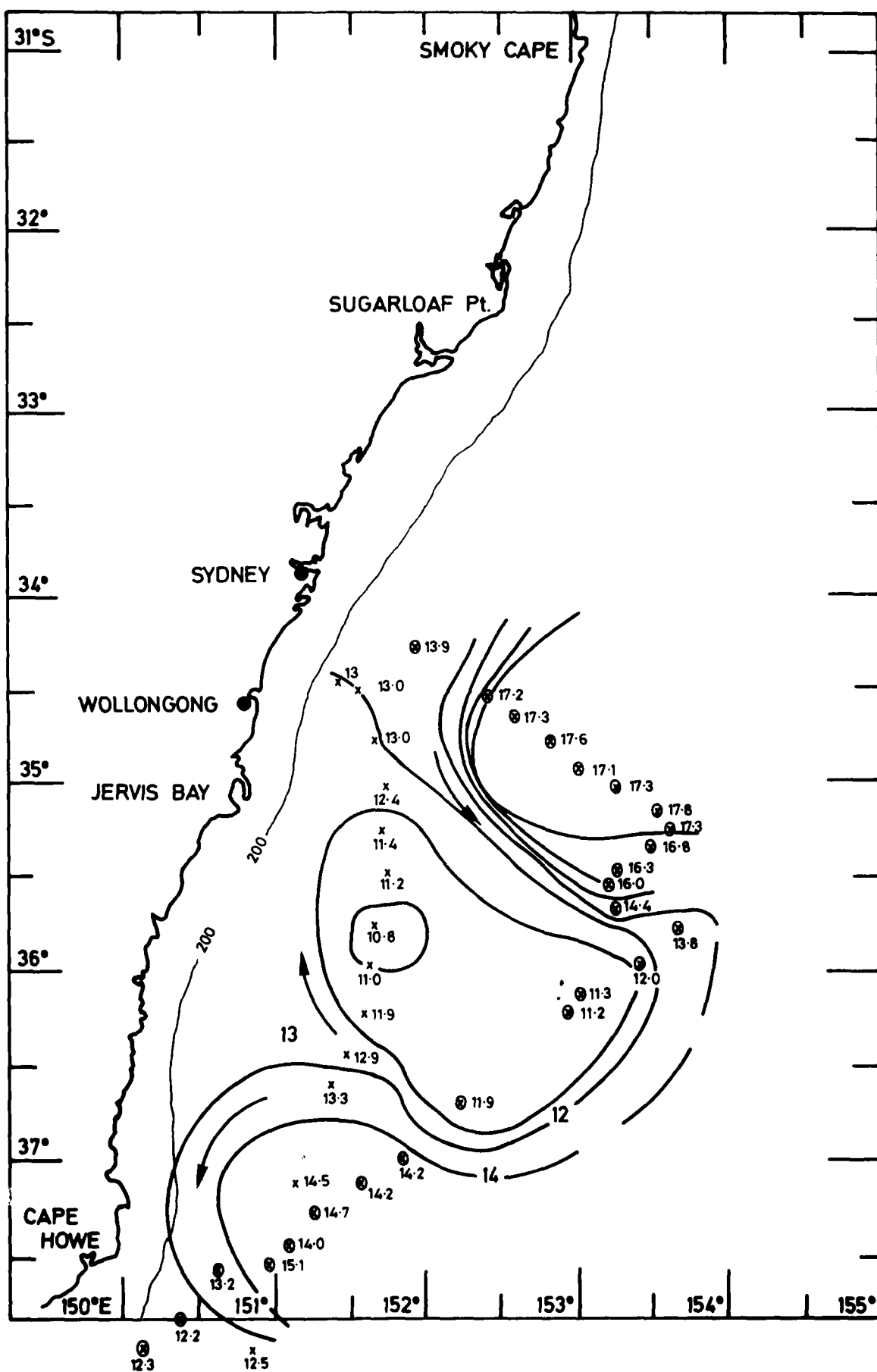
Fig. 24. T_{250} x 28-29 Oct. • 8-10 Nov.
