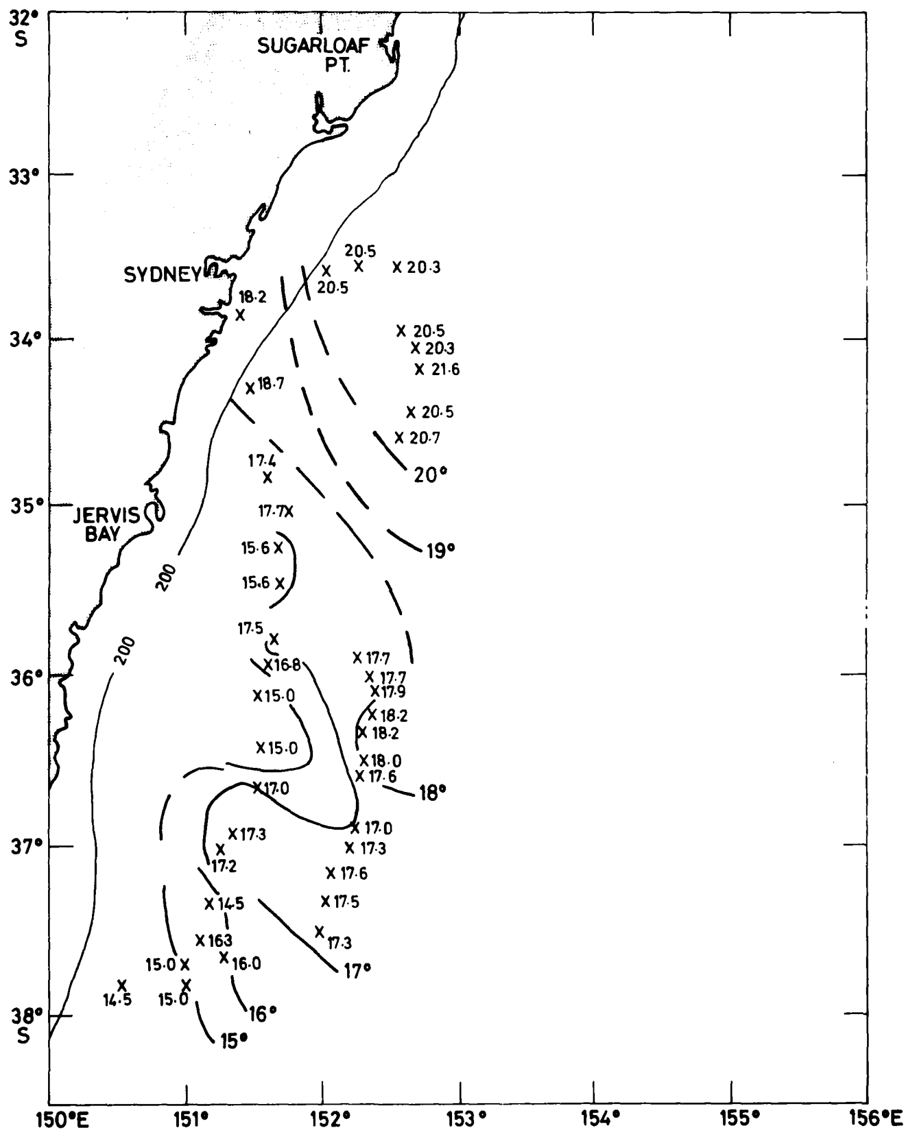
Fig.13. SST. 14-19 September 1981 from Kimbla (°C)
