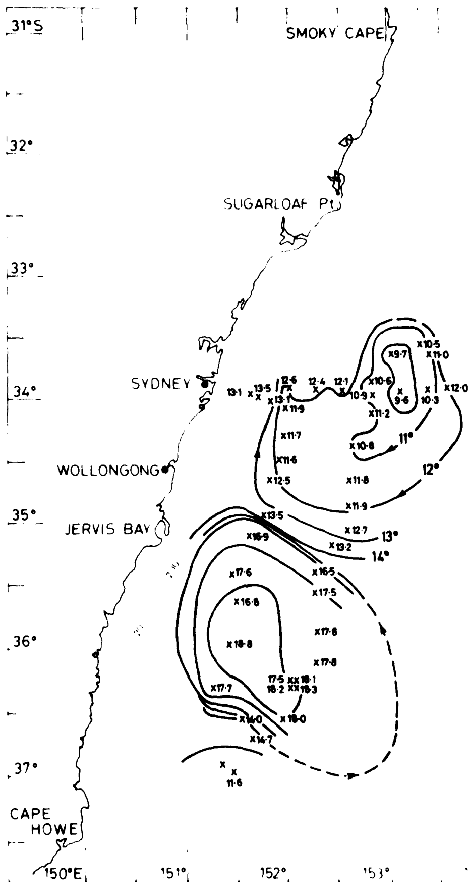
Fig. 6. T250 from Kimbla 11-15 March (°C)
