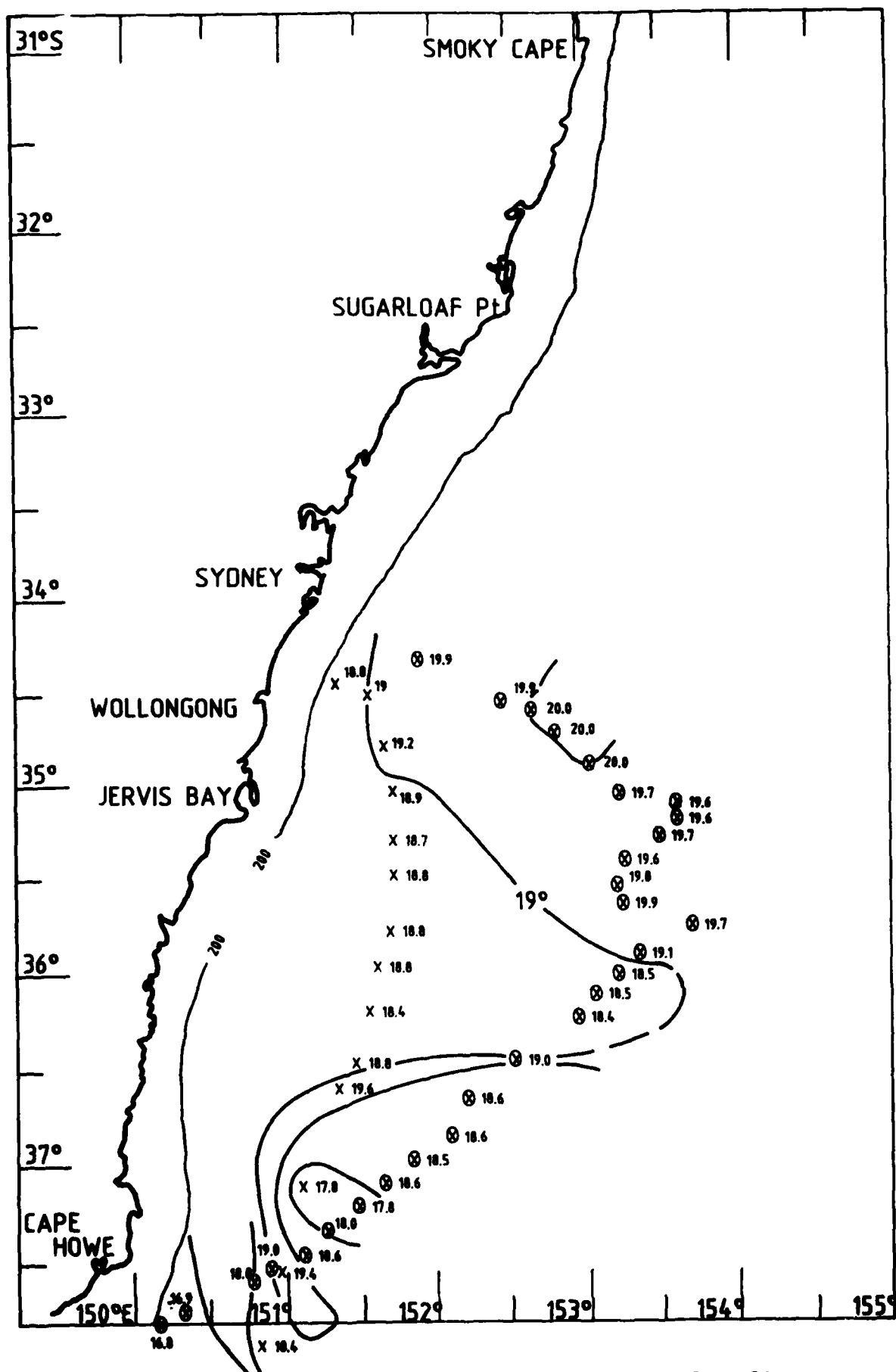
Fig. 22. SST from Kimbla x 28-29 Oct. 81 o 8-10 Nov. 81.
