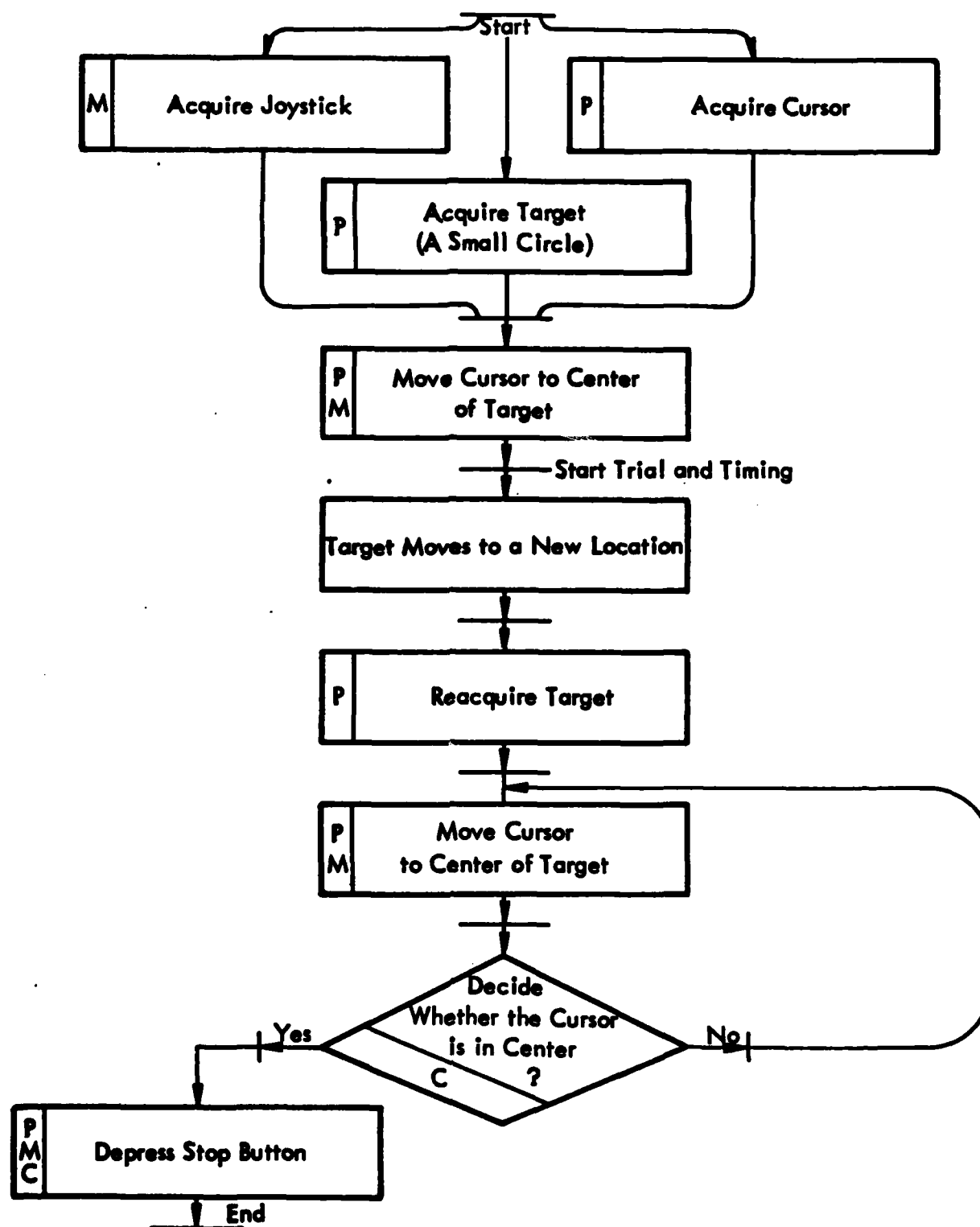
Figure B.18 Positioning using joystick and trackball. (Applies to all configurations.)
