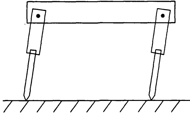
Figure 5-1: The model has five rigid links and four springy joints. The length of the legs can change, as can the angle of the legs with respect to the body. The links all have mass and moment of inertia.
