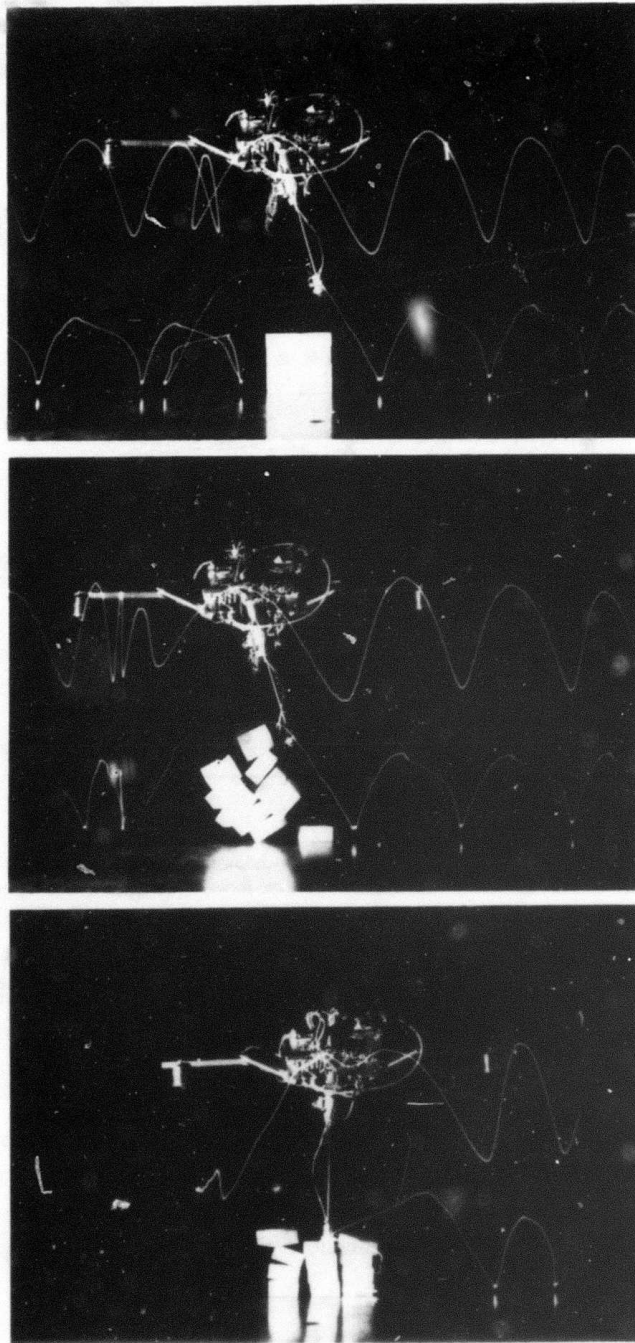
Figure 7-12: Planar one-legged system leaping. In order to successfully leap over an obstacle, a legged system must place its foot in the correct location with respect to the obstacle. The correct foot placement in the top photograph was a matter of good luck. In the middle photograph the foot was too close to the stack of blocks when the leap began, and the foot did not clear. The bottom photograph depicts a leap in which the takeoff point was too far from the obstacle. In all photographs action is from right to left, with lines indicating paths of foot and hip.
