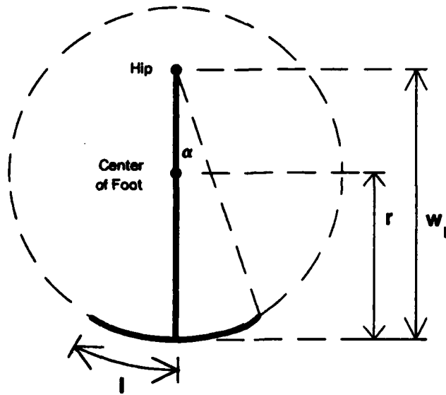
Figure 7-11: The foot can be an arc of a circle of radius, r . The angle subtended by the foot is \alpha .
