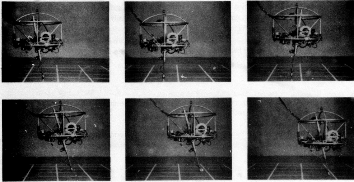
Figure 2-2: Sequence of photographs showing one complete stride of the 3D hopping machine running from left to right. Grid on floor indicates 0.5 m intervals. Running speed is about 1.75 m/sec, with stride length 0.63 m, and stride period 0.380 sec. Adjacent frames separated by 76 msec.
