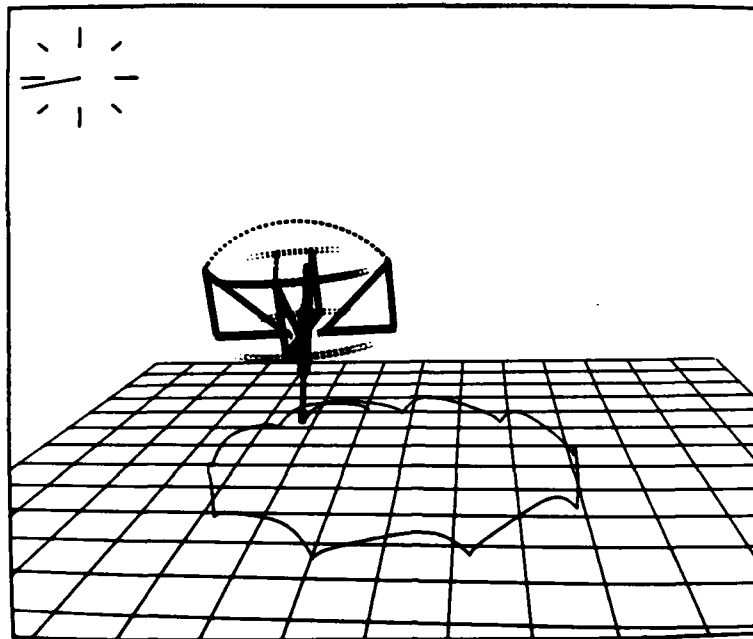
Figure 1-5: Simulated 3D one-legged machine running in circles. A constant lateral offset of the foot coupled with constant forward velocity, produces a constant radius of curvature.
