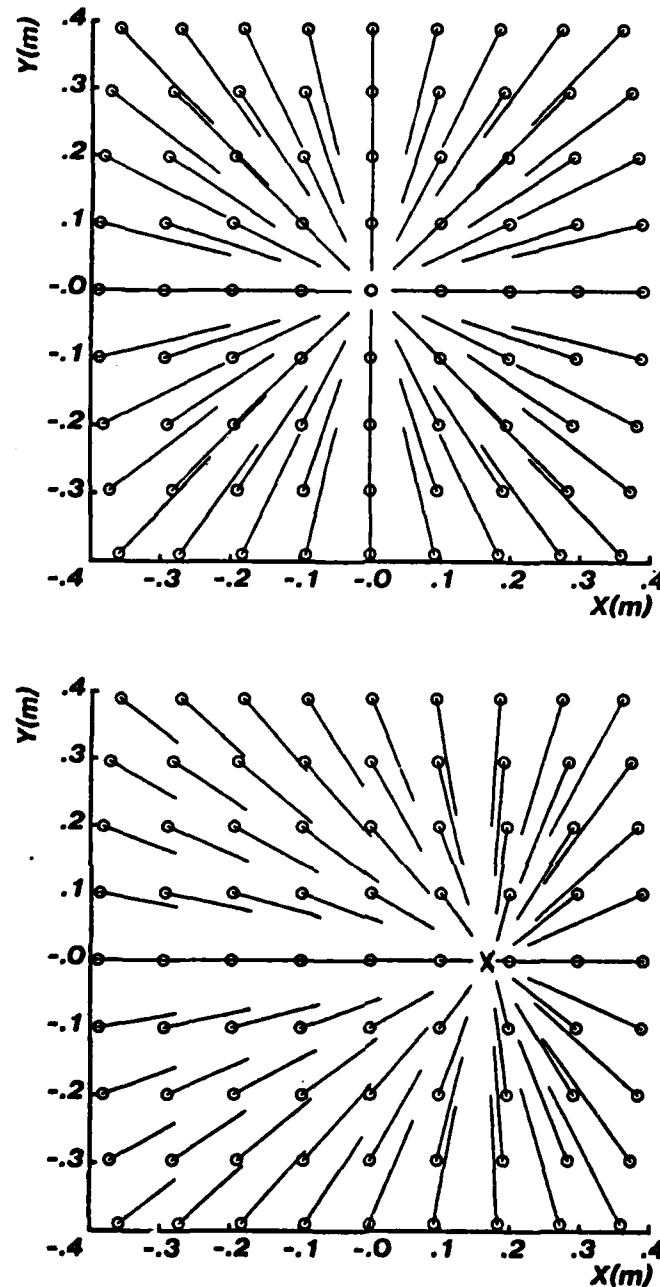
Figure 6-3: Effect of foot placement on the velocity of the hopper. The circles mark the position of the foot with respect to the center of gravity of the hopper at touch-down. The vectors represent the change in the velocity of the hopper for each foot placement during the stance phase. In the top figure the hopper has no forward velocity at touch-down. The acceleration vectors all point towards the origin. The length of the vectors increases with the distance from the origin. In the bottom figure the forward velocity at touch-down is 1 m/sec in the positive x direction. The x marks the foot placement that results in zero velocity change. The acceleration vectors point in this general direction. For small displacements the magnitude of the acceleration vectors increases with the distance from this point.
