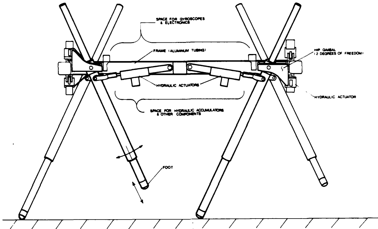
Figure 1-3: Diagram of machine under construction for experiments on balance in multi-legged systems that run. The machine will be about 1.0 m long, 0.6 m tall to the hip, and will weigh 35 kg. It is roughly the size and shape of a large dog.
