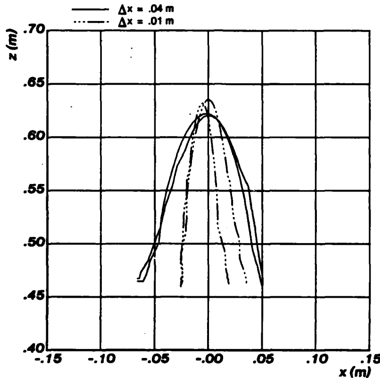
Figure 7-5: Position of center of mass of physical 3D hopping machine using pairs of balanced steps. The control algorithms were those described in Chapter 2, but an offset, \Delta x , was added to the foot position on even hops, and subtracted on odd hops. The magnitude of \Delta x is set to two different values. The body moved back and forth on alternate hops. The system was not stable during a single hop, but only over a pair of hops. This experiment is relevant to running gaits that do not place the effective point of support under the body, such as the pace and bound. The displacements of the foot, \pm x , correspond to the displacement of the hip from the center of the body. The trot and kangaroo hop do not involve such offsets.
