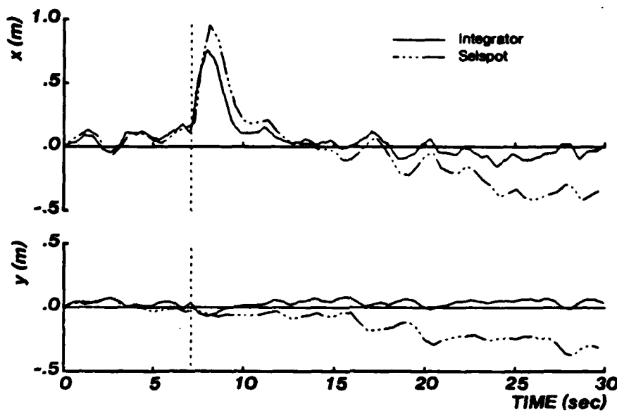
Figure 2-8: 3D machine hopping in place under position control. The control system integrated forward velocity to determine the machine's position in the room. An electro-optical system (Selspot) mounted on the ceiling provided an independent measurement of the machine's position. Divergence between Selspot and integrator data indicates drift in the integrator. DOTTED LINE: Experimenter disturbed the machine by delivering a sharp horizontal jab to the frame with his hand. It returned to the position setpoint within a few seconds. (3D.332.4)
