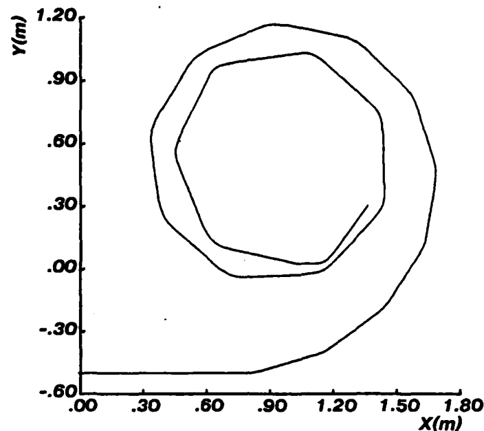
Figure 6-5: Spiral Trajectories. The lateral acceleration during the stance phase increases with the lateral displacement of the foot. If the displacement is increased each successive hop, then the hopper follows a spiral trajectory. Here the forward speed was fixed at 0.6 m/sec. D_{Lat} was increased from 0.0 to 0.035 m.
