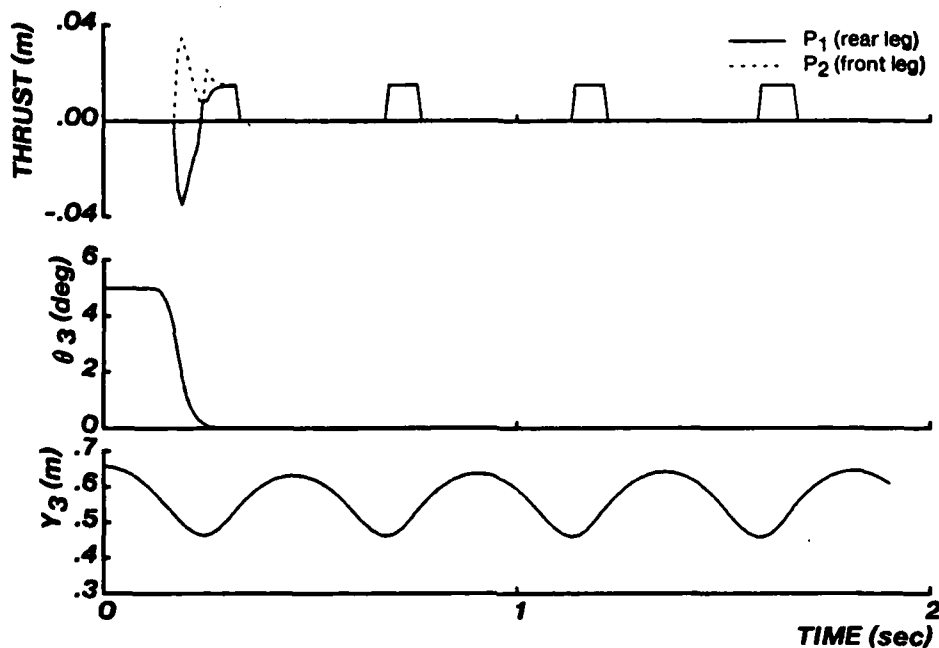
Figure 3-4: Hopping with attitude control. Differential leg thrust corrected an error in body attitude. A constant leg thrust maintained hopping height. During the first cycle, the body angle was driven to zero by the differential thrusting. On the remaining steps, thrusting maintained the vertical amplitude. The graph of thrust shows the change in the length of the position actuator of each leg which was proportional to the active thrust.
