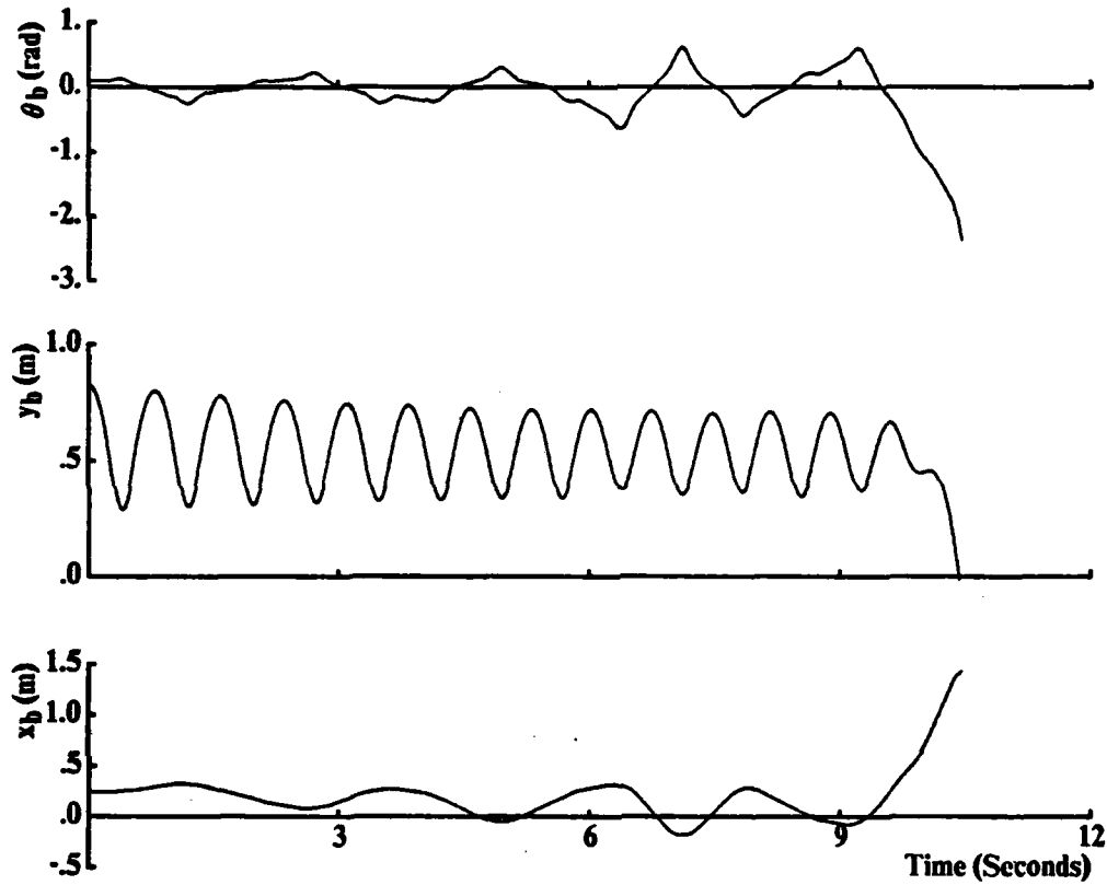
Figure 5-7: Unlike the graphs in Fig. 5-5, these graphs are from a simulation where periodic motion was not established. (Simulation r.323.5)
