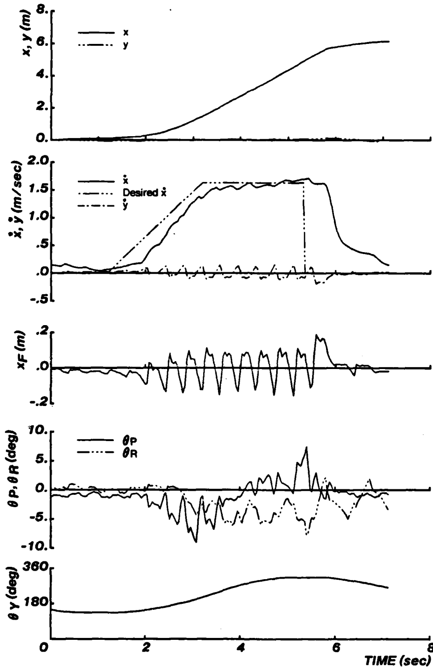
Figure 2-6: Velocity control was examined by varying the desired velocity in the x direction from 0. to 1.6 m/sec with an acceleration of 1 m/sec 2 , then holding the setpoint constant for about 2 seconds, and then setting the rate setpoint to zero. (Dashed line in second plot.) Facing direction of the body, \theta_Y , was measured but not controlled. Also shown are TOP: the position of the machine in the room, MIDDLE: the position of the foot with respect to the hip, BOTTOM 2: and the yaw orientation of the body. (3D.335.12)
