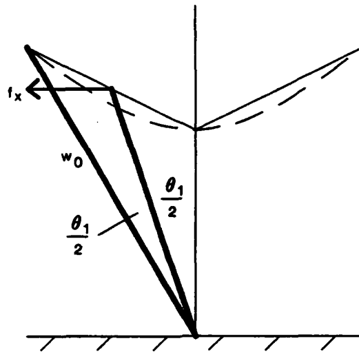
Figure 7-15: Diagram that shows straight-line approximation to the path of the body during stance. Also shown is the point at which the backward force exerted by the leg on the body is approximately equal to the average backward force for the first half of stance.
