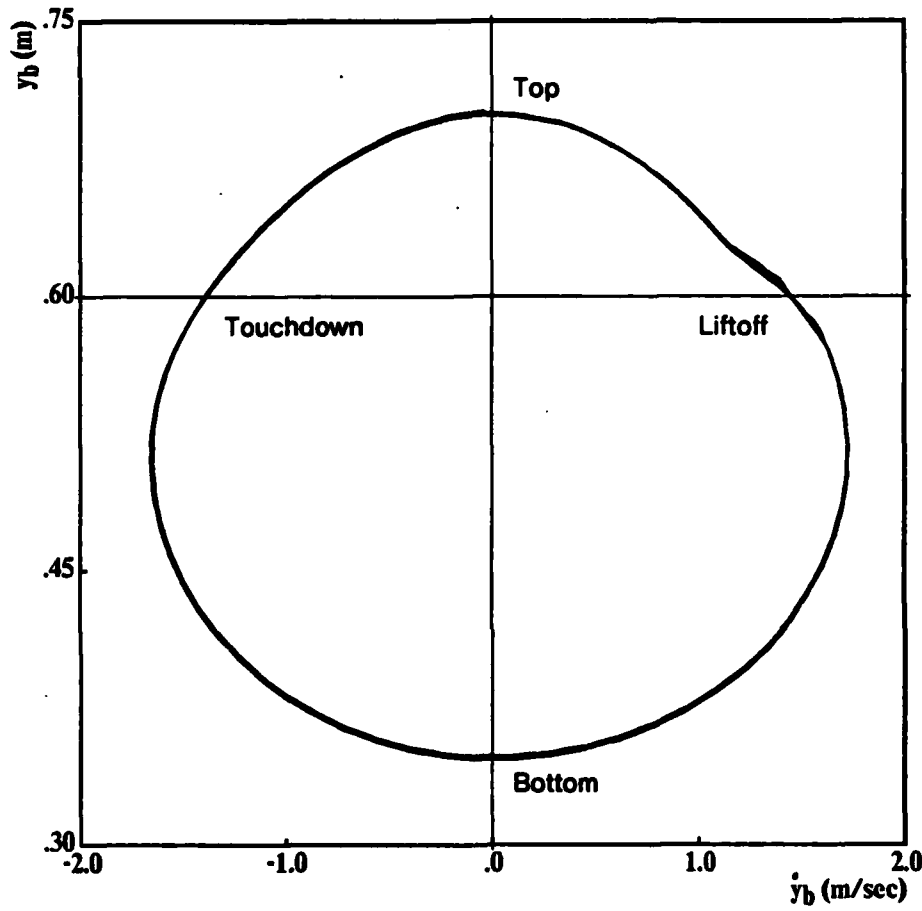
Figure 5-4: The vertical position of the center of gravity of the body is plotted along the vertical axis, and the vertical velocity along the horizontal axis. The upper part of the plot is parabolic, the motion of a body experiencing the constant acceleration of gravity. The lower part is harmonic, the motion of a spring mass oscillator. Note the notch caused by the impact of the stops against the lower legs. This phase plot is from simulation r.319.8 and shows several cycles of vertical bouncing. The model parameters are listed in Appendix B.
