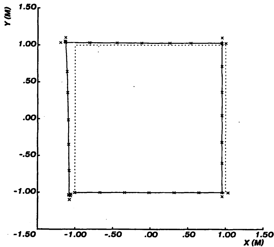
Figure 6-1: Path control. The 3D model was made to follow a square path. It started at (-1,-1), lower left, and progressed anti-clockwise through (1,-1), (1,1), and (-1,1), finally returning to the starting point. Total time around the square was 24 sec.
