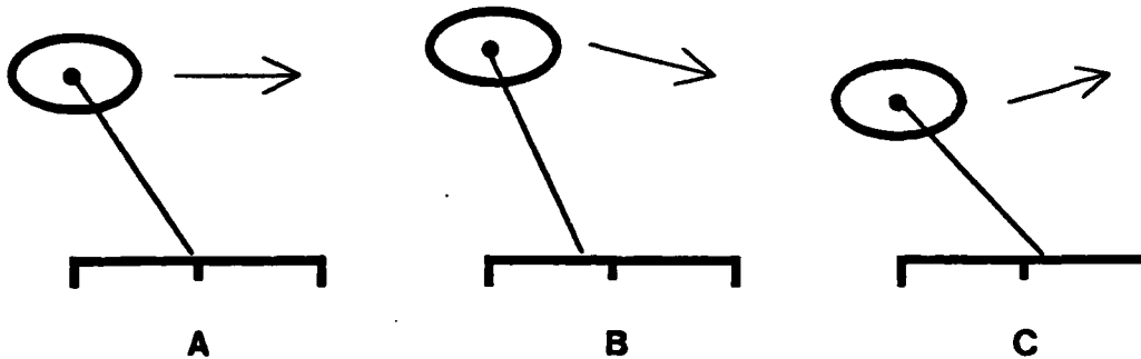
Figure 2-4: Behavior when foot is displaced from the center of the CG-print. A: When foot is placed in the center of the CG-print the system tips neither forward nor backward, and it does not change its forward running velocity. B: When foot is placed toward the rear of CG-print, the body tips and accelerates forward during stance. C: When foot is placed toward the front of CG-print, the body tips backward and decelerates during stance. Horizontal lines indicate the CG-print for each case.
