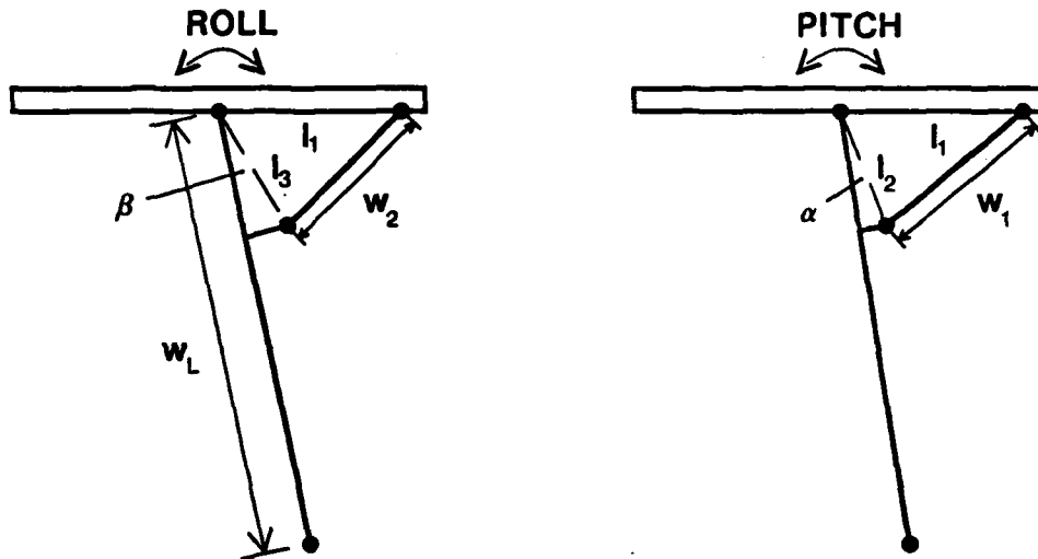
Figure 2-11: Diagram that shows kinematics of actuators, hip, and leg. Actuator lengths are represented by w_1 and w_2 , and leg length by w_L . l_1=0.345 m, l_2=0.0508 m, l_3=0.0762 m, \alpha=8.46 deg, \beta=27.28 deg.
