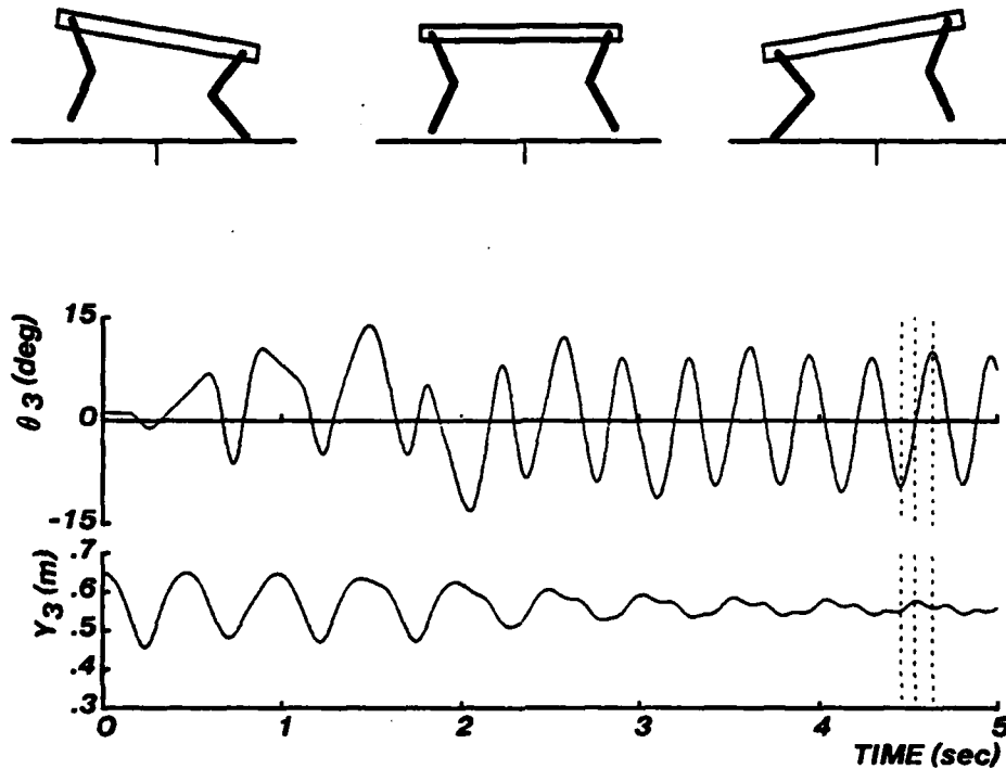
Figure 3-6: Hopping without active attitude control. Each leg thrusts independently when its hip reached bottom. A constant thrust was used. The desired velocity was set to zero. At first there was a random pattern, but it was soon replaced by a stable pattern of bouncing from one foot back onto the other. The center of gravity remained nearly stationary while the body pitches back and forth.
