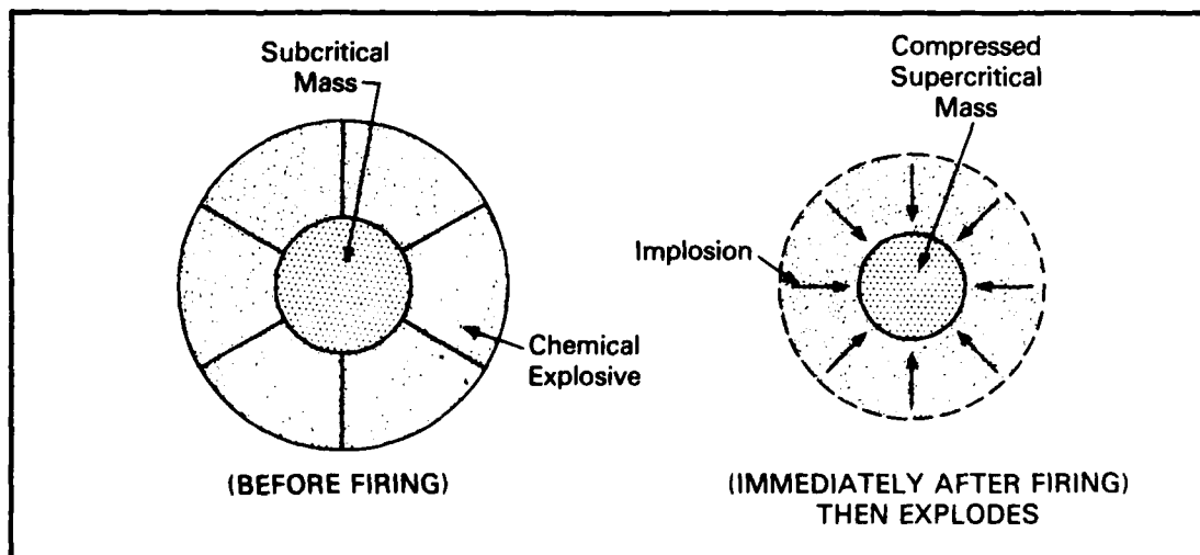
Figure 1-1b: PRINCIPLE OF IMPLOSION-TYPE NUCLEAR DEVICE (GLASSTONE AND DOLAN)
