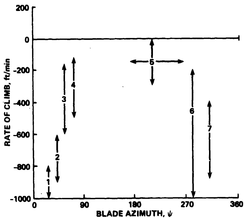
Figure 7.- Flight conditions for potential blade-vortex interactions.
