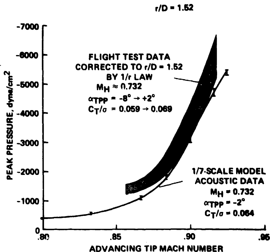
Figure 31.- Peak negative-pressure amplitude comparison: full-scale and model-scale high-speed data.
