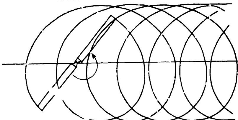
Figure 68.- Epicycloidal tip-vortex pattern for \mu = 0.164 .
