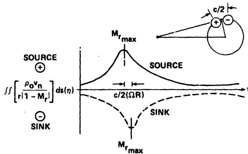
Figure 3.- Variation of M_r over observer time.
