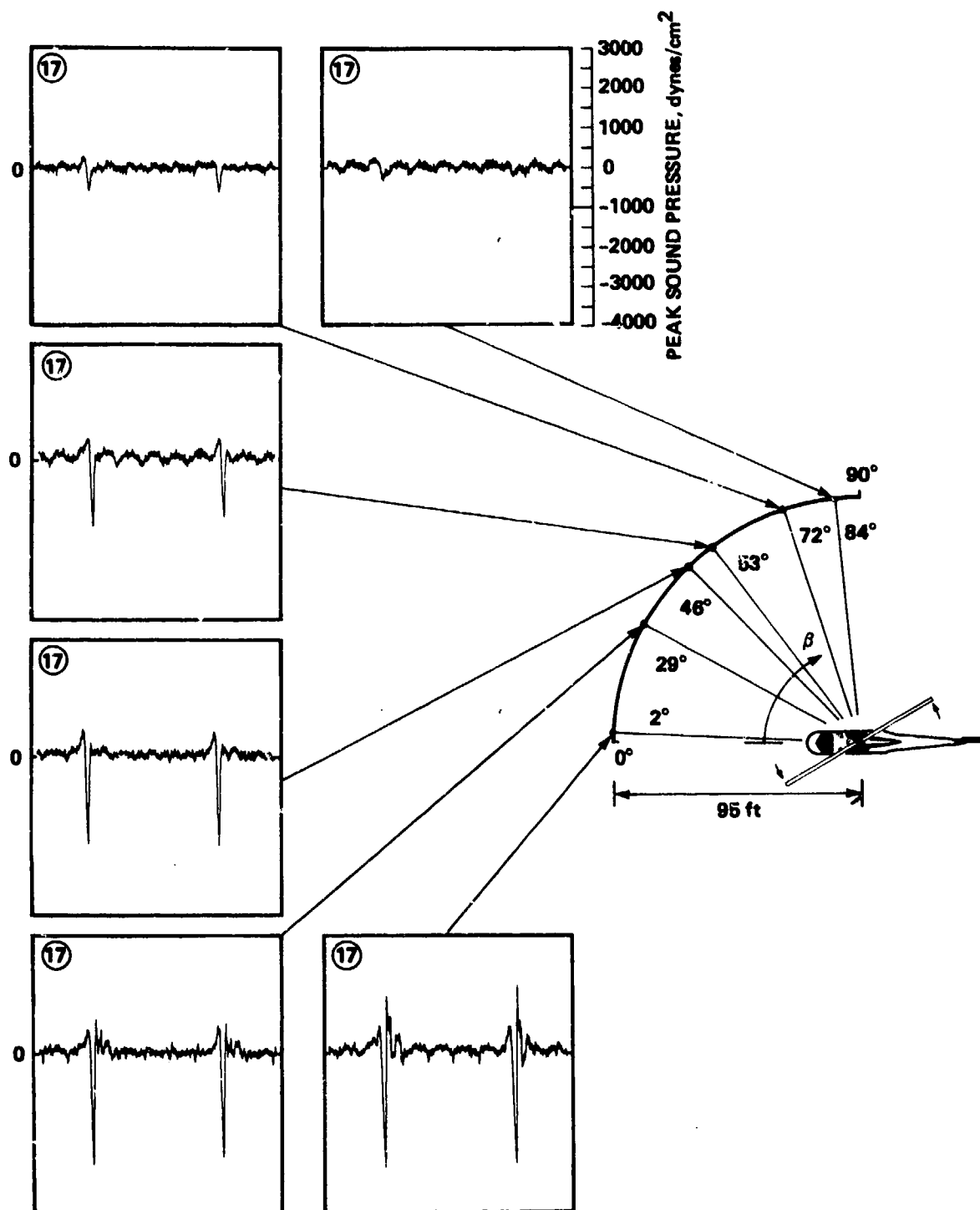
Figure 21.- UH-1H lateral acoustic directivity, level flight, 115 kncts IAS ( \alpha = 7^\circ ).
