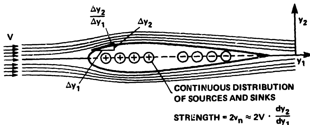
Figure 46.- Monopole acoustic sources.
