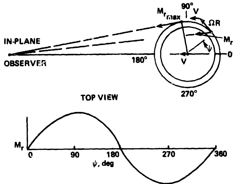
Figure 2.- Variation of M_r over azimuthal angles.
