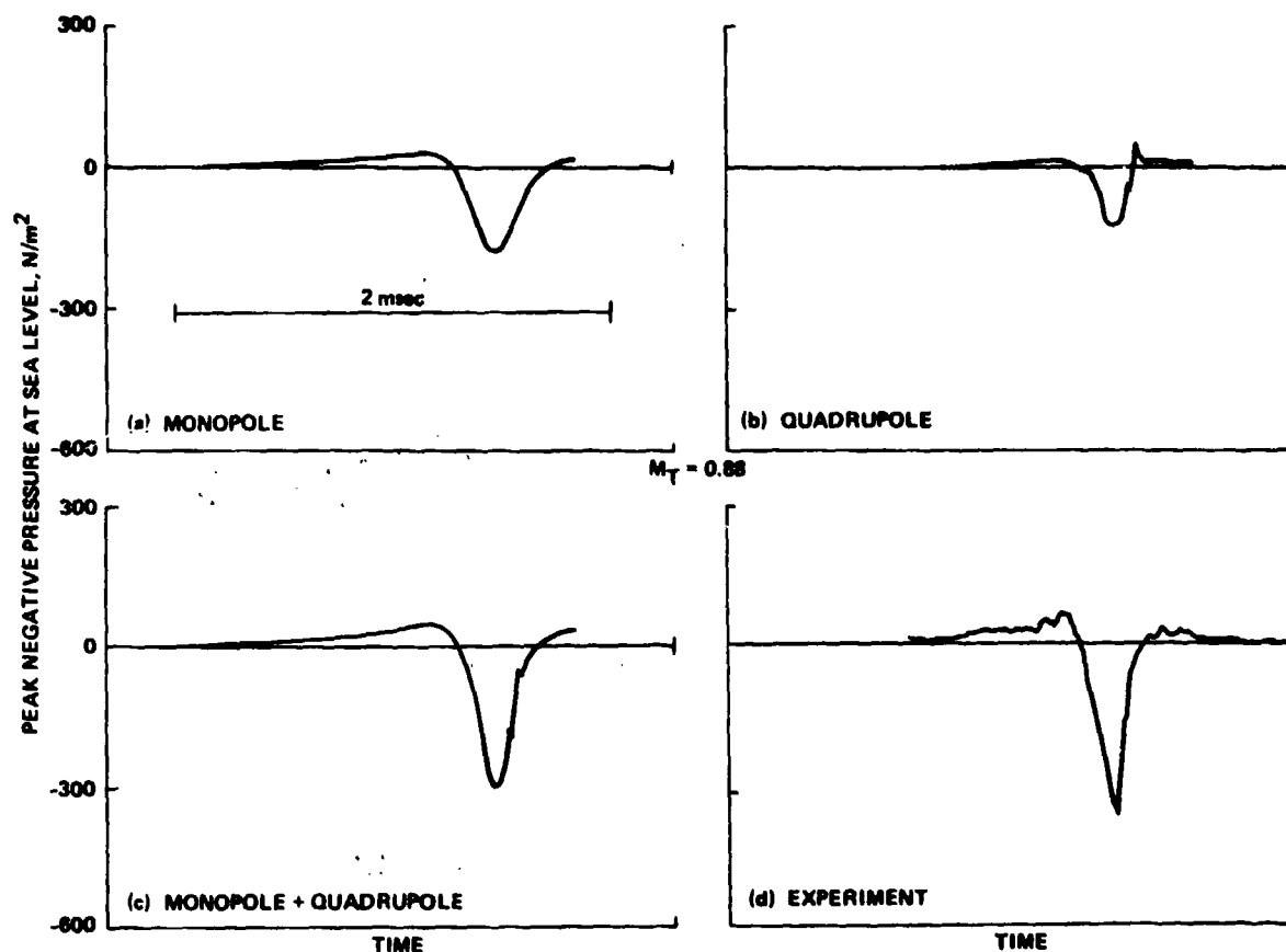
Figure 62.- Theory-experiment comparison, M_T = 0.88 .
