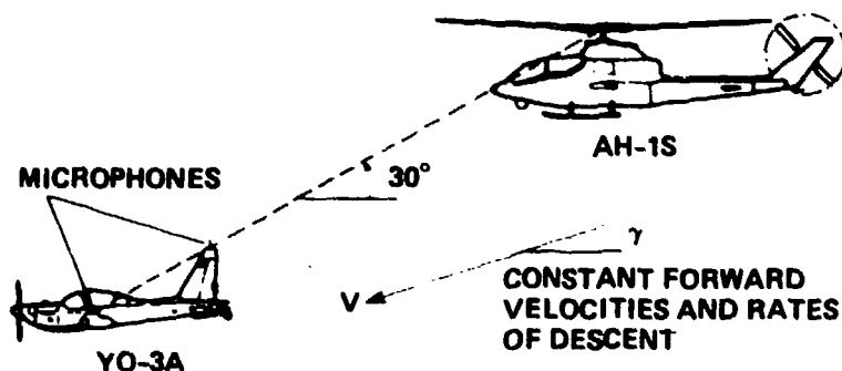
Figure 66.- Full-scale blade-vortex interaction acoustic measurement technique.
