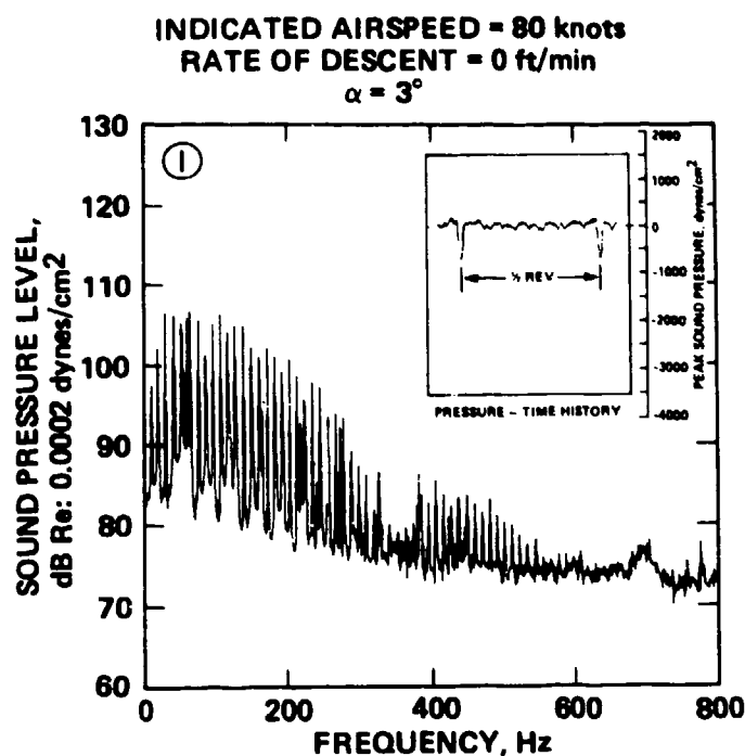
Figure 25.- In-plane UH-1H acoustic power spectrum for level flight, 80 knots IAS: \alpha = 3^\circ , \beta = 0^\circ .
