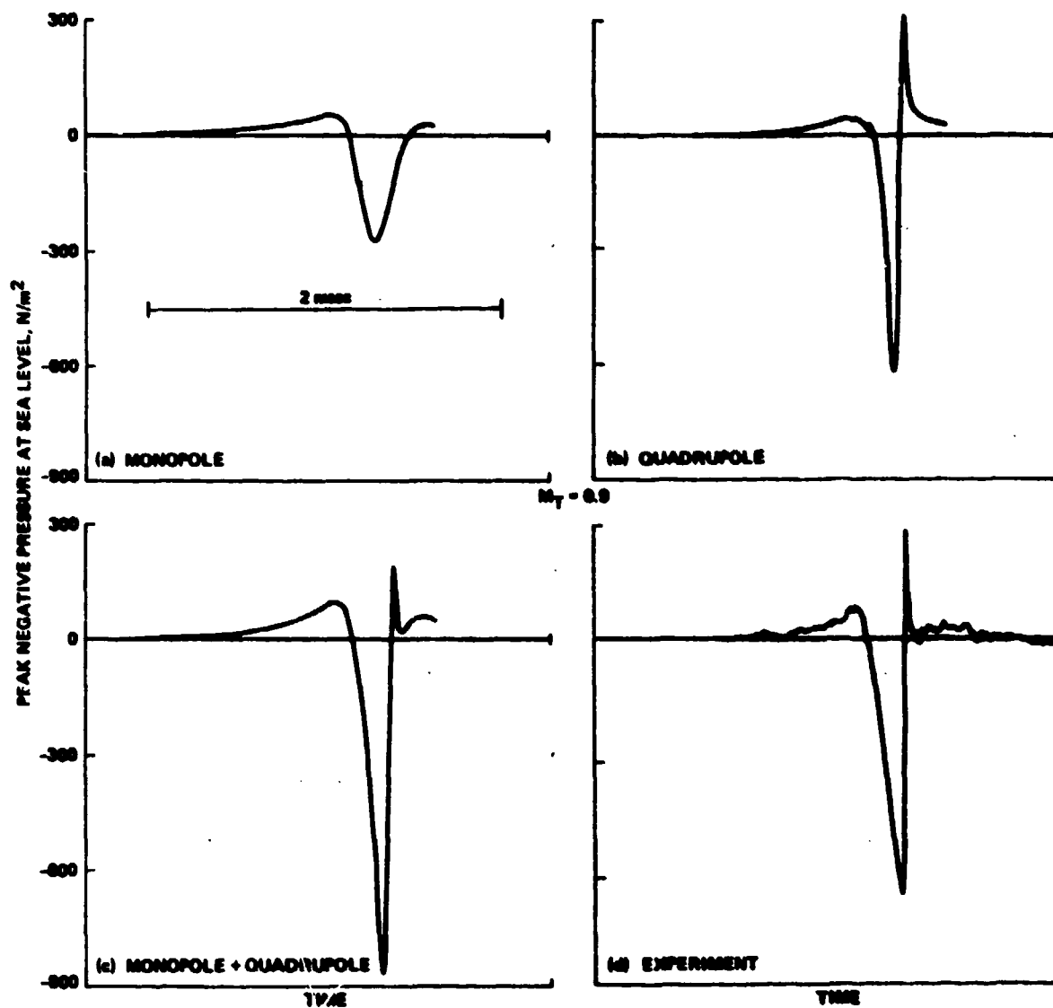
Figure 63.- Theory-experiment comparison, M_T = 0.90 .
