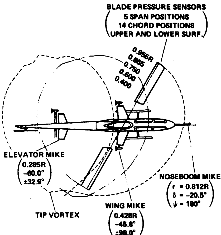
Figure 73.- Simultaneous measurement of blade surface-pressure and noise.
