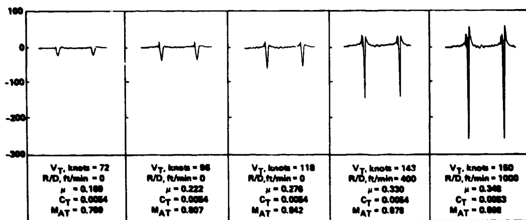
Figure 32.- Comparison of model and full-scale acoustic pressure for an in-plane microphone 1.8 rotor diameters ahead.
