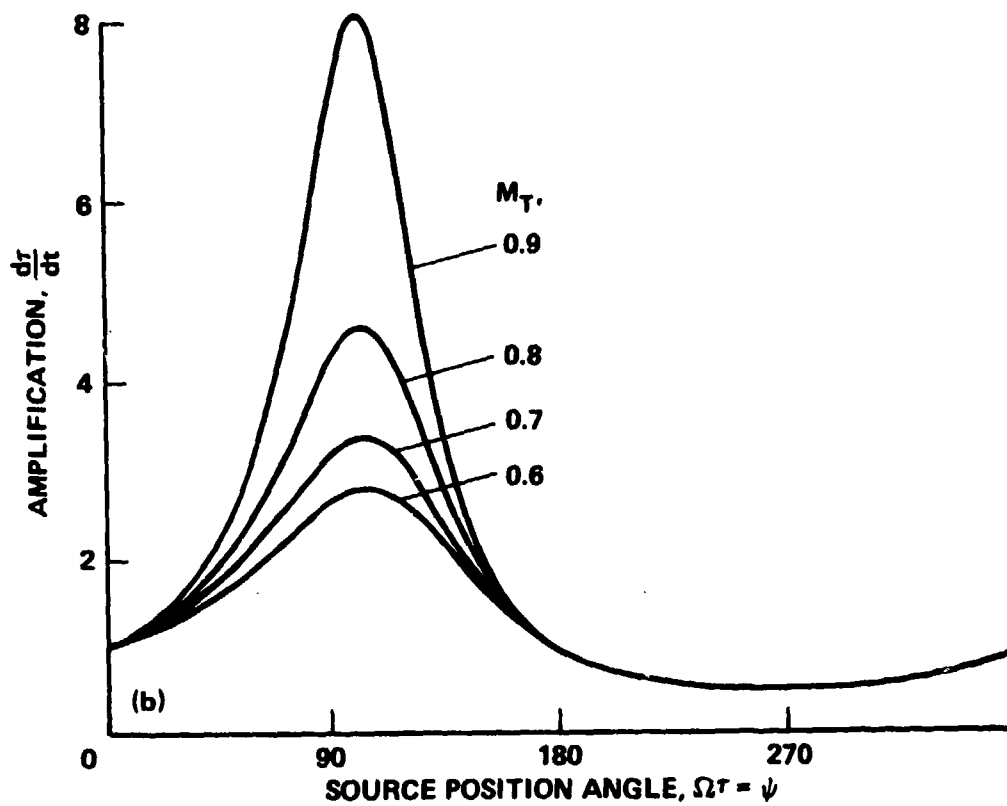
Figure 48.- Retarded time factor.
