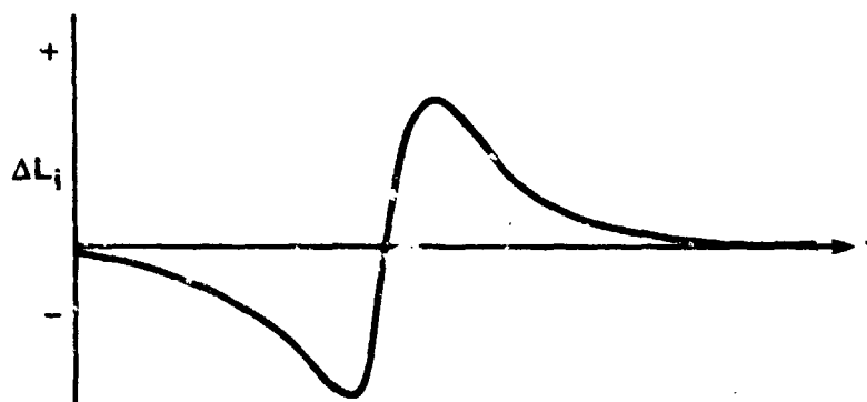
Figure 10.- Lift history of an advancing blade.
