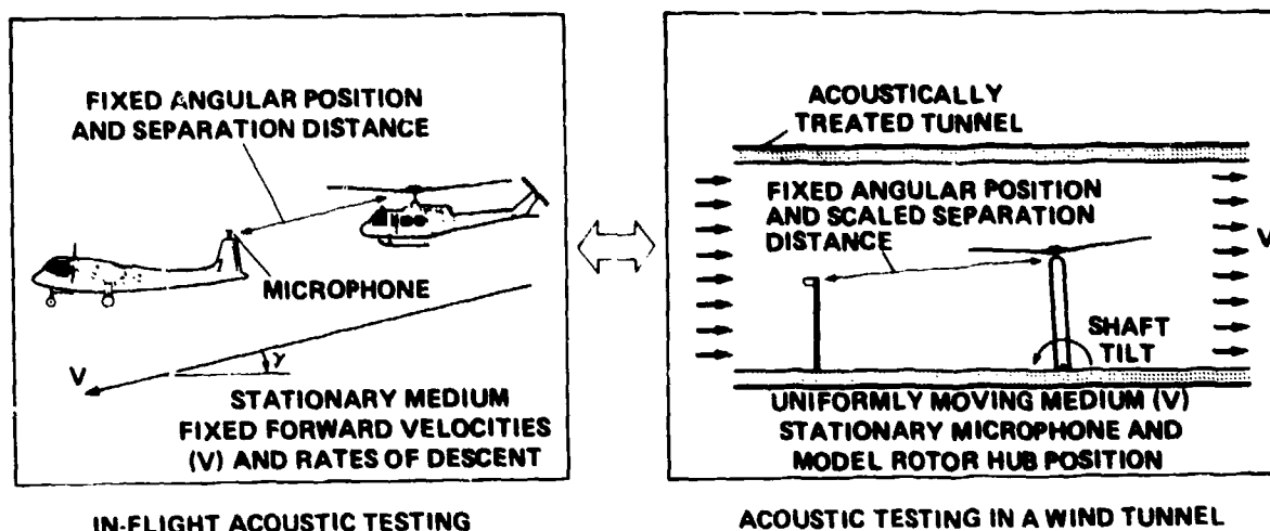
Figure 29.- Model and full-scale acoustic testing.
