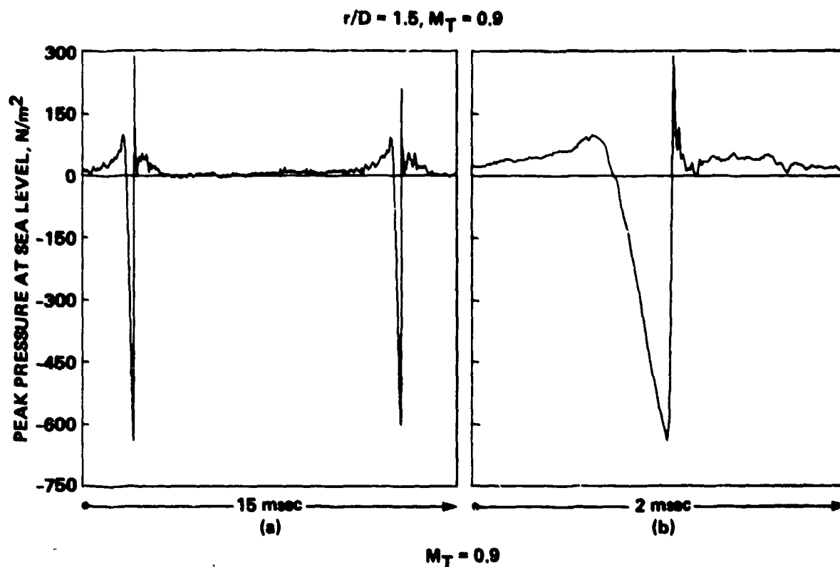
Figure 42.- Acoustic pressure time-history, in plane, r_H/D = 1.5 , M_T = 0.9 .
