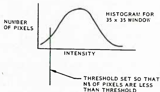
Figure 35. Thresholding. 19
