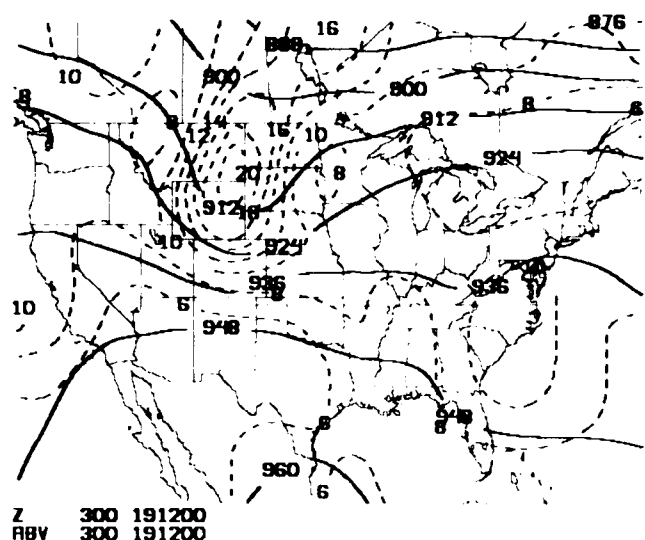
Figure C8. 300-mb Heights (solid, decameters) and 300-mb Absolute Vorticity (dashed, \times 10^{-5} \text{ sec}^{-1} )
