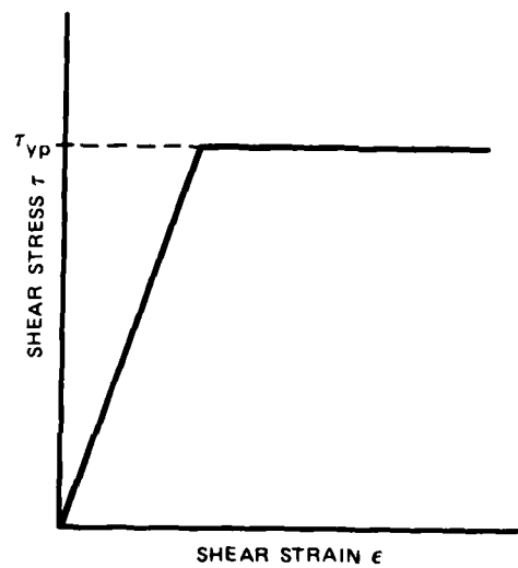
b. PERFECT ELASTIC-PLASTIC MATERIAL
