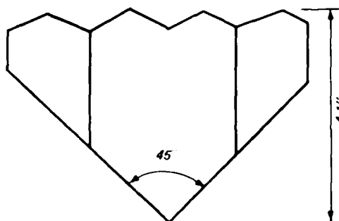
Figure 16. Shape of IC direct shear specimen
