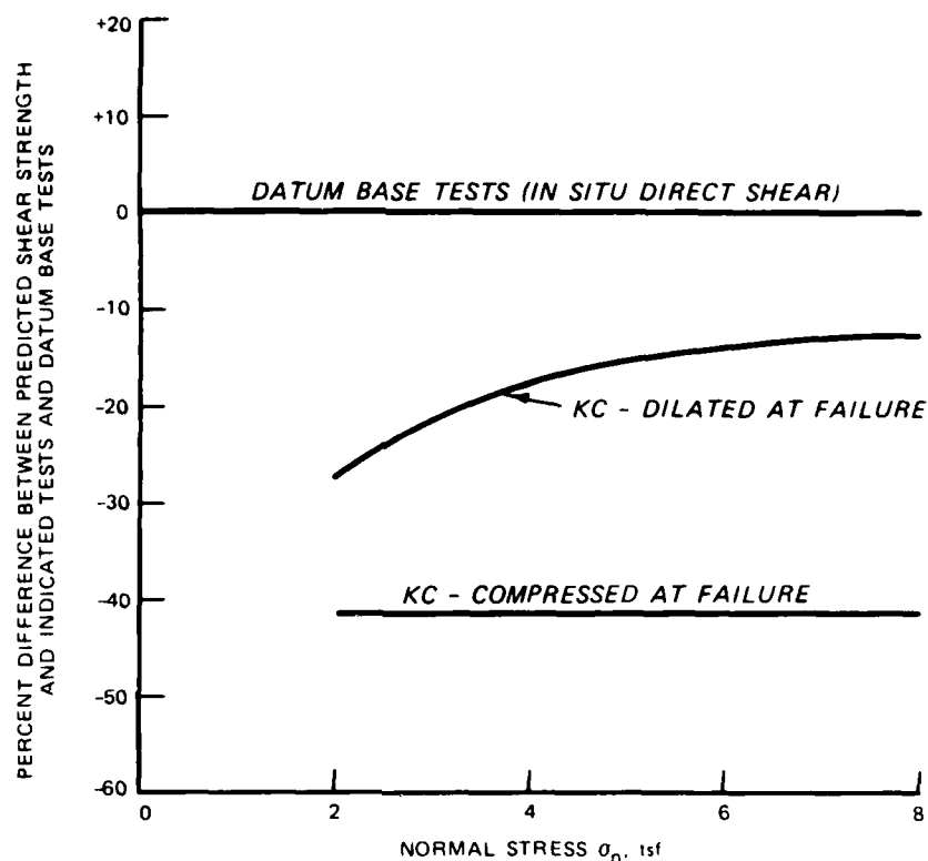
Figure 74. Normal stress versus percent difference between predicted shear strength from indicated tests and datum base tests on Rangely sandstone natural joint specimens
