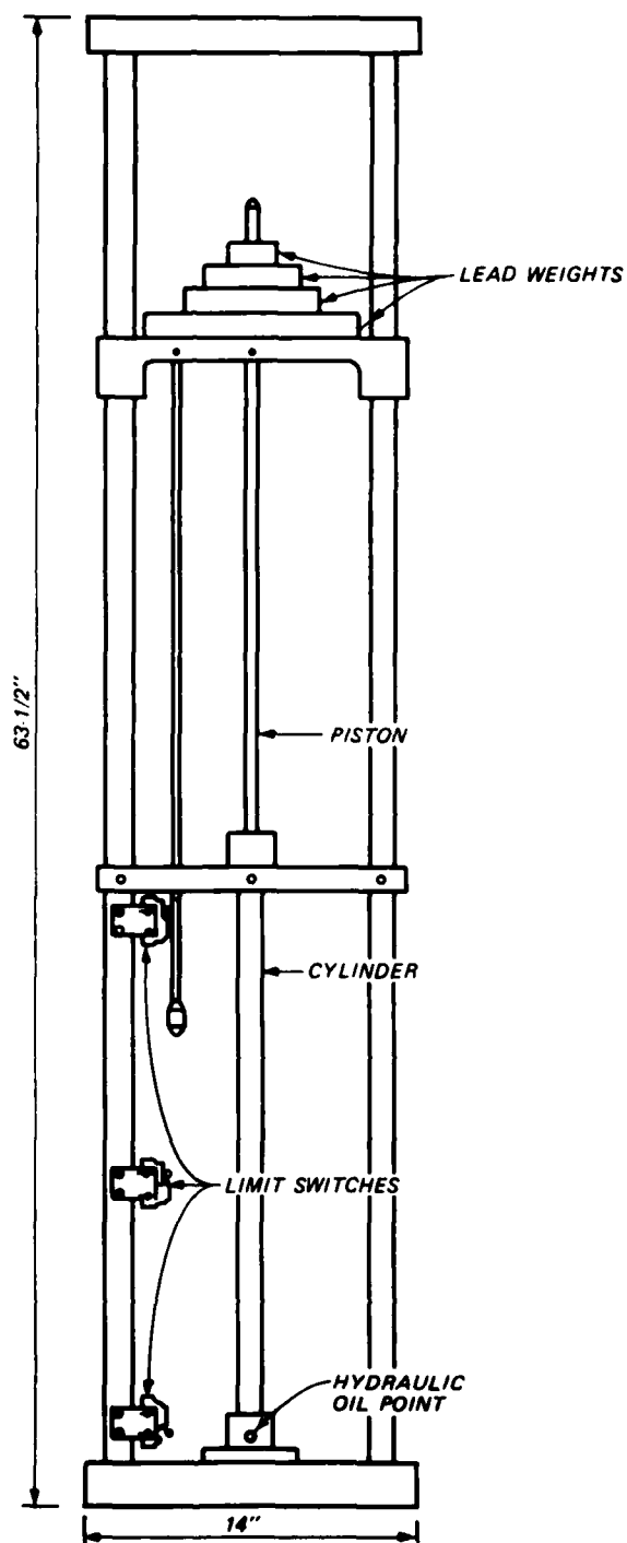
Figure 3. Deadweight normal load system
