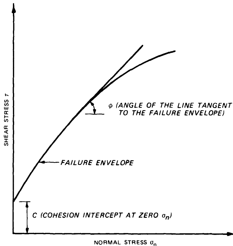
Figure 17. Hypothetical failure envelope
