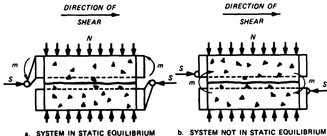
Figure 54. Schematic of typical direct shear devices
