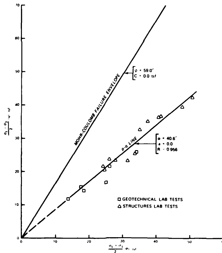
Figure 63. Composite p-q diagram of GL and SL triaxial tests on model material intact specimens
