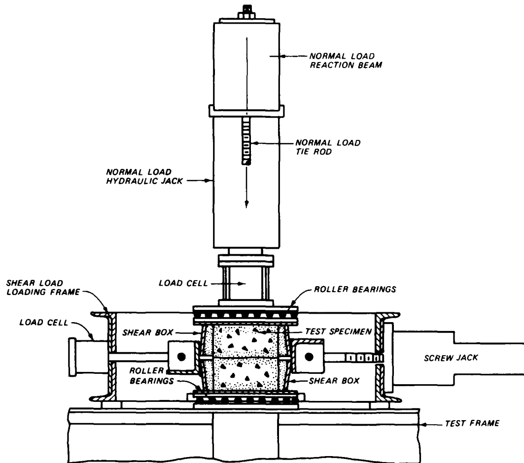
Figure 10. Schematic of KC direct shear device
