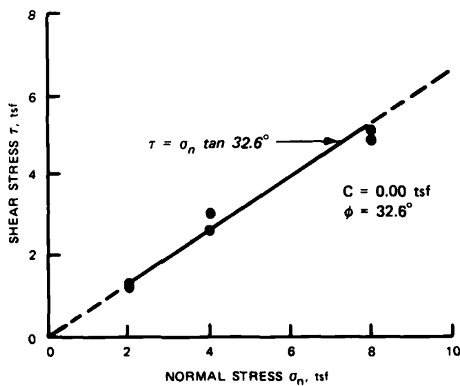
Figure 51. Three- by three-inch direct shear test results for smooth sawn Rangely sandstone specimens
