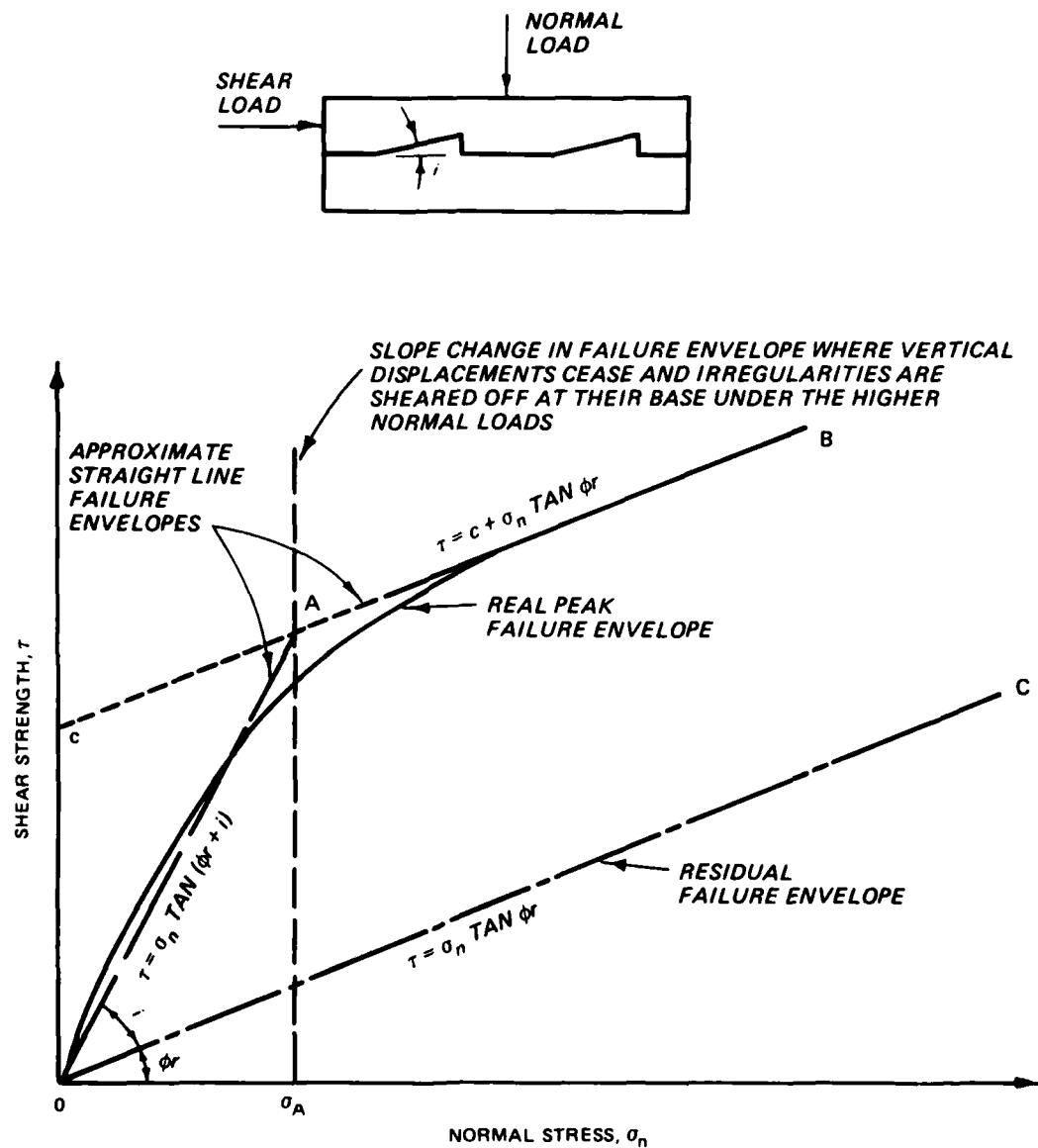
Figure 22. Maximum and residual strength failure envelope from tests of discontinuities (after Deere et al., 1967)
