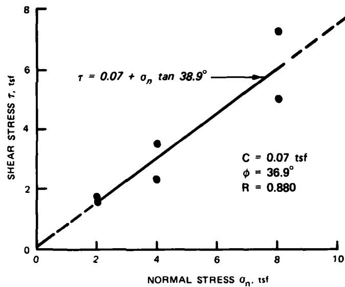
Figure 50. KC direct shear test results for Rangely sandstone natural joint specimens
