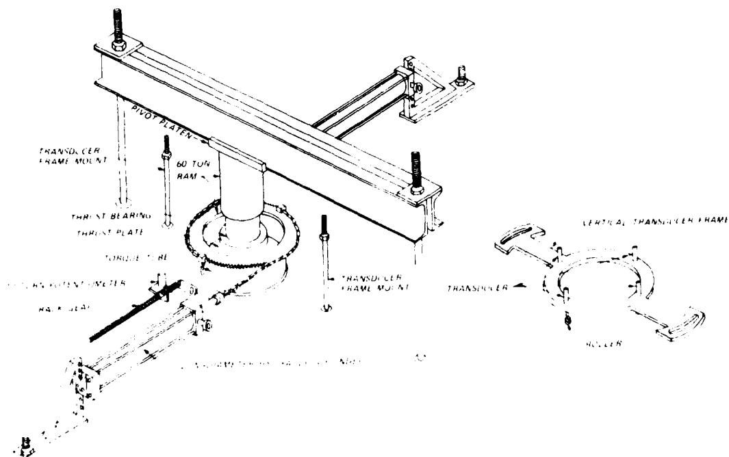
Figure 7. In situ torsional shear device
