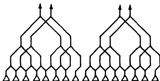
(c) SELECTION-CONSTRAINED 16-TO-4 NETWORK (Discrete Type) S = 36, L = 4, P = 28
