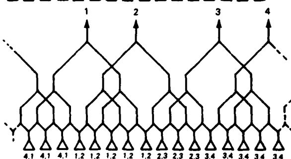
(d) SELECTION-CONSTRAINED 16-TO-4 NETWORK (Merged Type) S = 44, L = 4, P = 32
