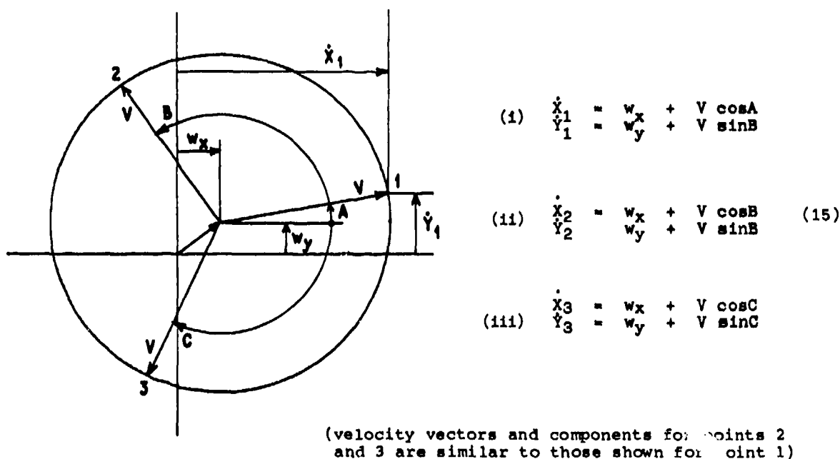
Figure 3 Velocity Vectors for Radar Speed Measurement
