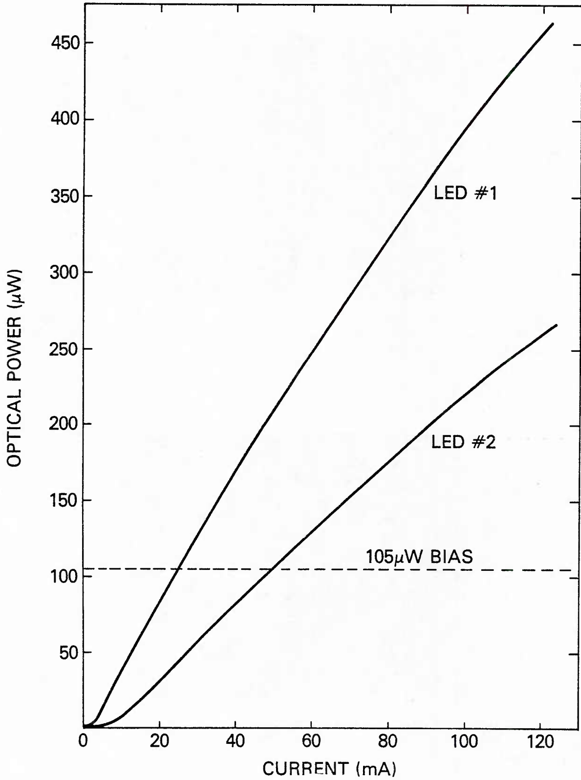
Fig. 13 — Optical transfer characteristics for the two LEDs.
