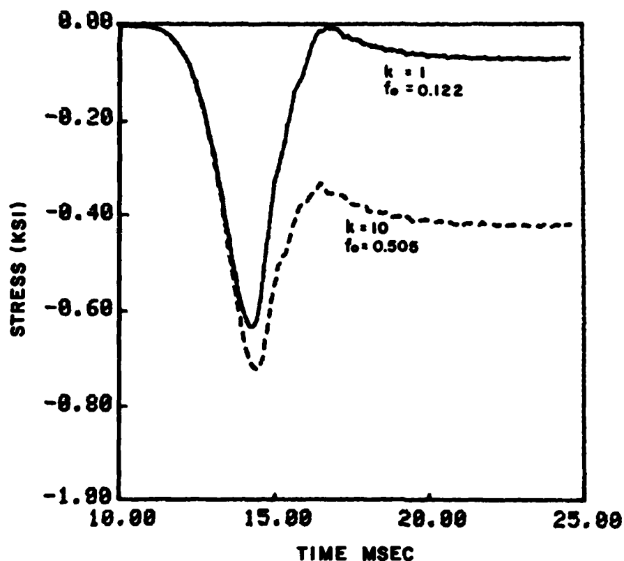
FIG. 13 STRESS HISTORIES AT 20.3 FEET FOR HYSTERETIC SOIL ( U_0 = 4 ) AND PLASTIC SHEAR SUPPORTS
