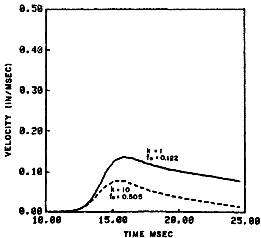
FIG. 14 VELOCITY HISTORIES AT 20 FEET FOR HYSTERETIC SOIL ( U_0 = 4 ) AND PLASTIC SHEAR SUPPORTS
