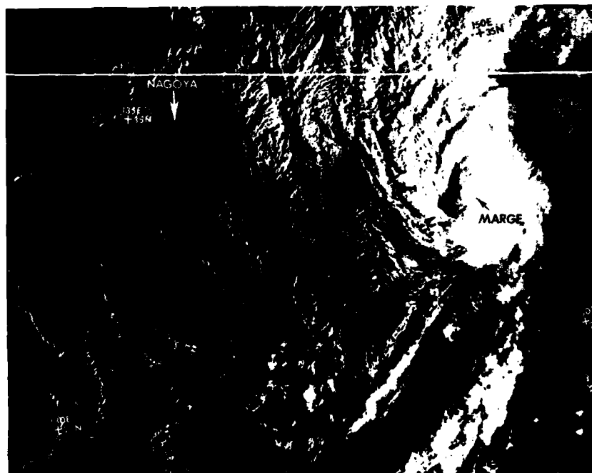
Figure 3-18-2. Marge just prior to completing transition to an extratropical system. Maximum sustained winds were 90 kt (46 m/s) and speed of movement was 51 kt (95 km/hr) (062254Z November NOAA 8 visual imagery).
