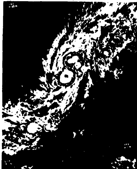
Figure 3-23-2. Tropical Storm Sperry at maximum intensity while undergoing an anticyclonic loop (031335Z December DMSP infrared imagery).
