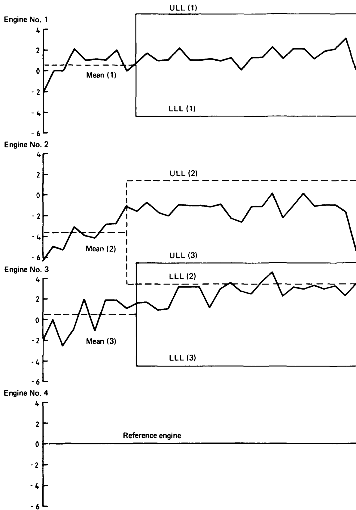
FIG 19 \Delta TORQUE – DIFFERENCE BETWEEN CORRECTED OBSERVED TORQUES, ENGINE NOS. 1-3 MINUS ENGINE NO. 4
